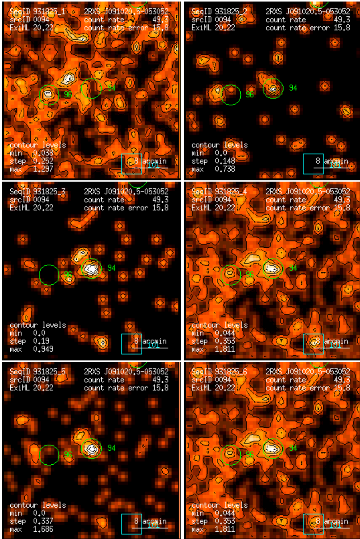
Figure 94: RASS 931825: detection 0094: band rate images, Gaussian filter: (1) PSPC channels 11 – 41, (2) 52 – 90, (3) 91 – 201, (4) 11 – 235, (5) 52 – 201, (6) 11 – 201. Broad band rates in counts/ks. Band rate contour levels in counts/ks/arcmin 2 .
