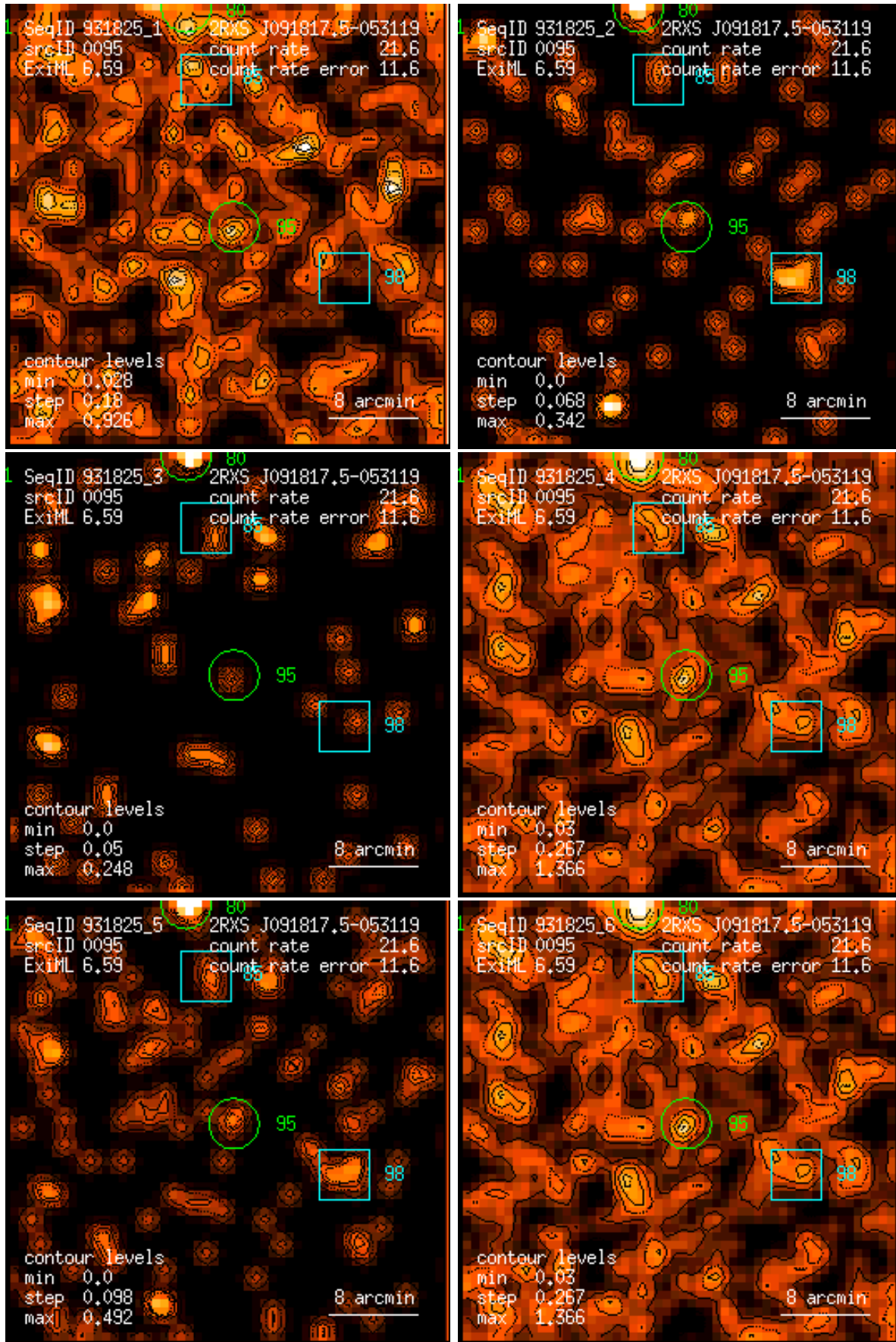
Figure 95: RASS 931825: detection 0095: band rate images, Gaussian filter: (1) PSPC channels 11 – 41, (2) 52 – 90, (3) 91 – 201, (4) 11 – 235, (5) 52 – 201, (6) 11 – 201. Broad band rates in counts/ks. Band rate contour levels in counts/ks/arcmin 2 .
