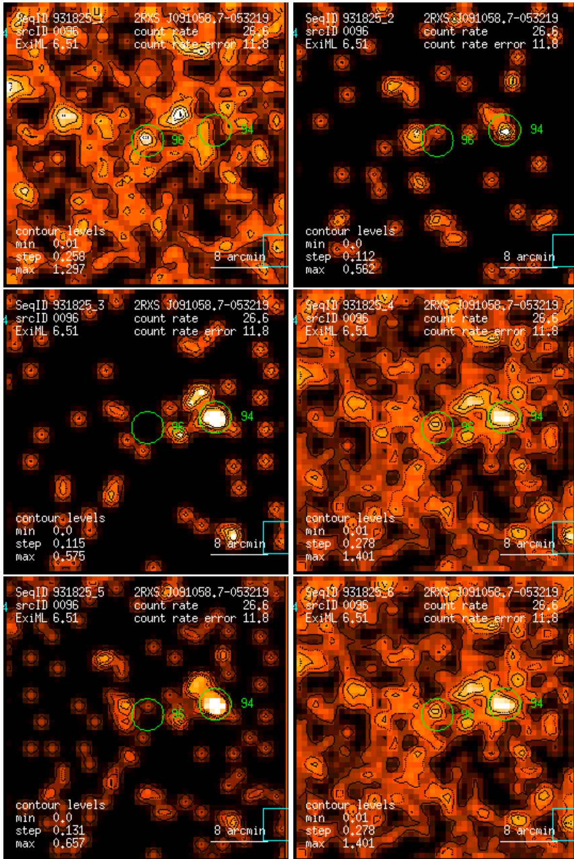
Figure 96: RASS 931825: detection 0096: band rate images, Gaussian filter: (1) PSPC channels 11 – 41, (2) 52 – 90, (3) 91 – 201, (4) 11 – 235, (5) 52 – 201, (6) 11 – 201. Broad band rates in counts/ks. Band rate contour levels in counts/ks/arcmin 2 .
