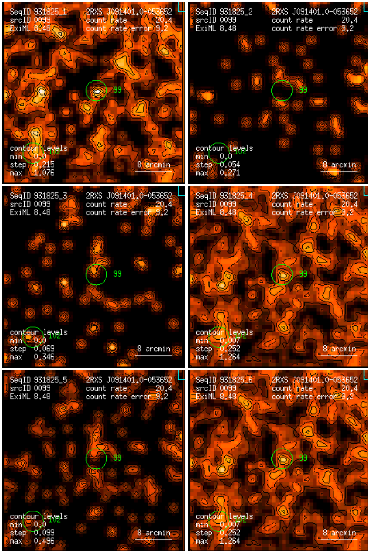
Figure 99: RASS 931825: detection 0099: band rate images, Gaussian filter: (1) PSPC channels 11 – 41, (2) 52 – 90, (3) 91 – 201, (4) 11 – 235, (5) 52 – 201, (6) 11 – 201. Broad band rates in counts/ks. Band rate contour levels in counts/ks/arcmin 2 .
