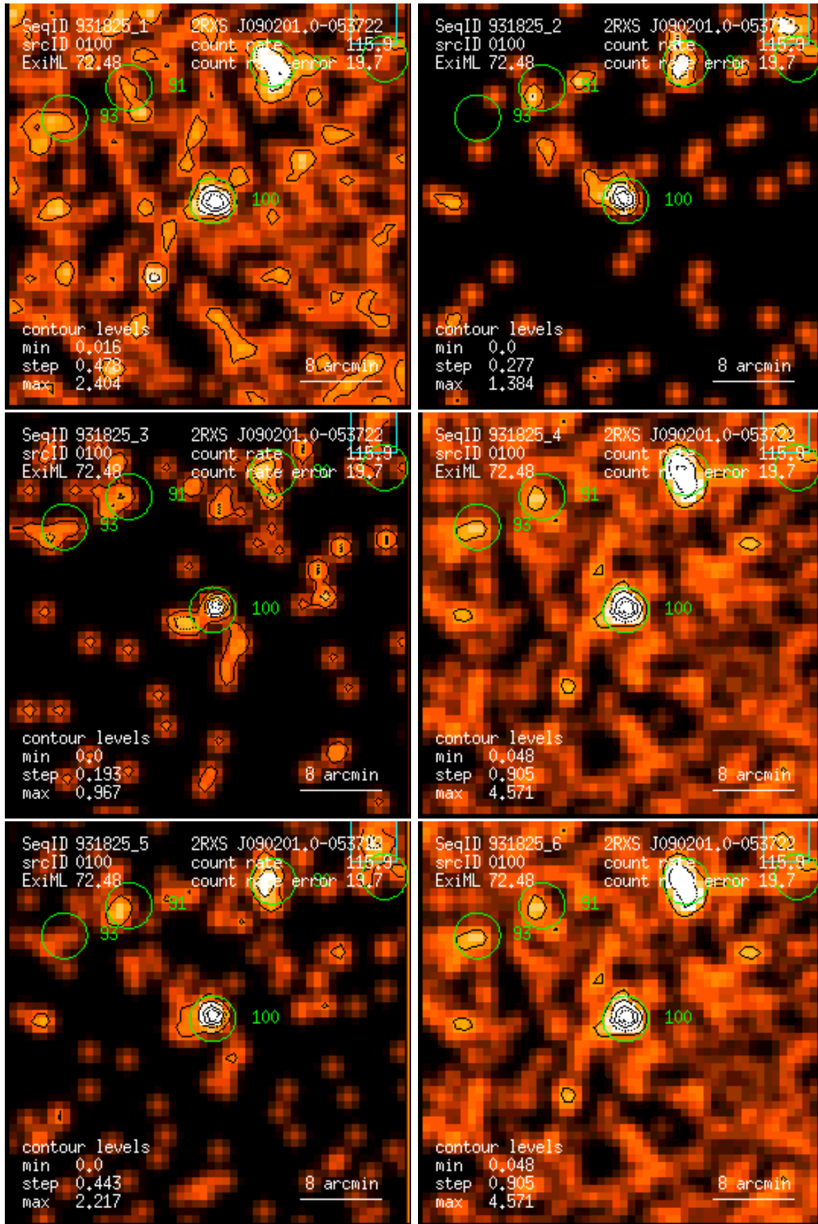
Figure 100: RASS 931825: detection 0100: band rate images, Gaussian filter: (1) PSPC channels 11 – 41, (2) 52 – 90, (3) 91 – 201, (4) 11 – 235, (5) 52 – 201, (6) 11 – 201. Broad band rates in counts/ks. Band rate contour levels in counts/ks/arcmin 2 .
