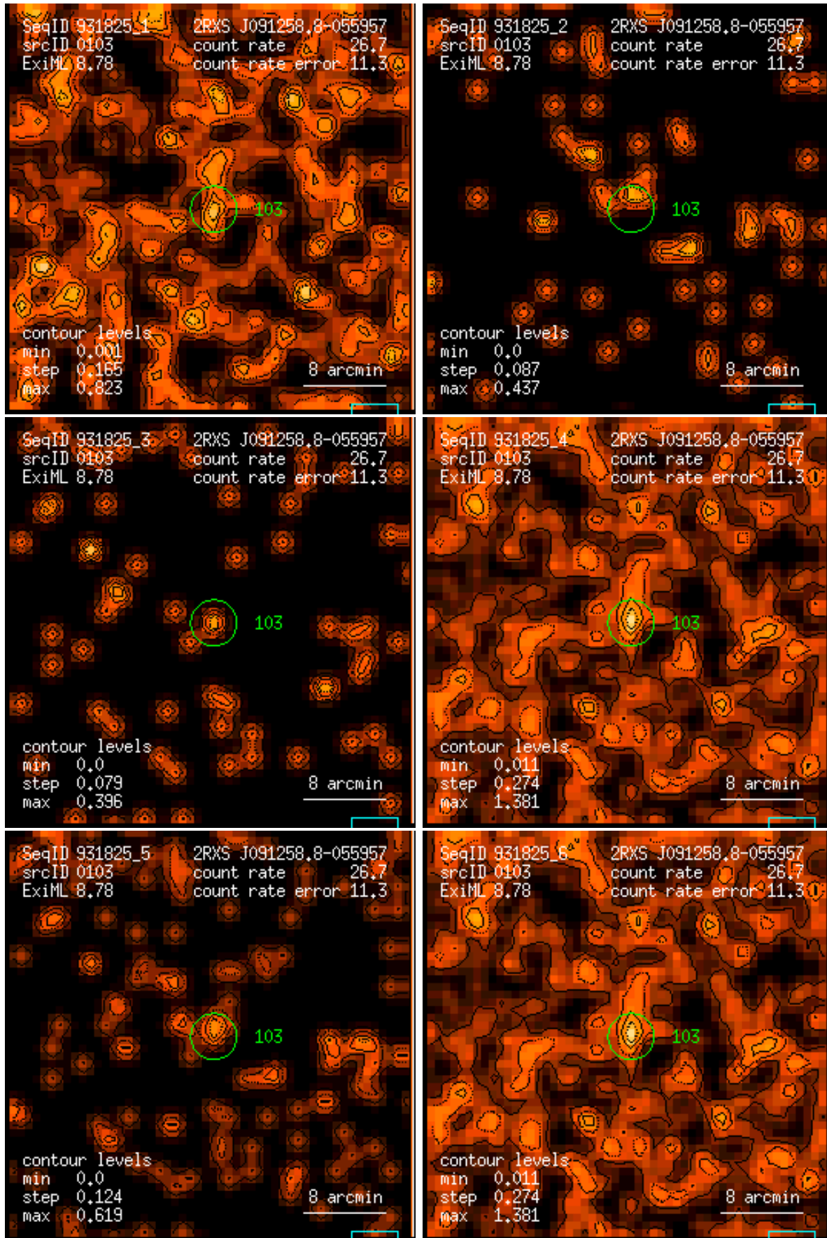
Figure 103: RASS 931825: detection 0103: band rate images, Gaussian filter: (1) PSPC channels 11 – 41, (2) 52 – 90, (3) 91 – 201, (4) 11 – 235, (5) 52 – 201, (6) 11 – 201. Broad band rates in counts/ks. Band rate contour levels in counts/ks/arcmin 2 .
