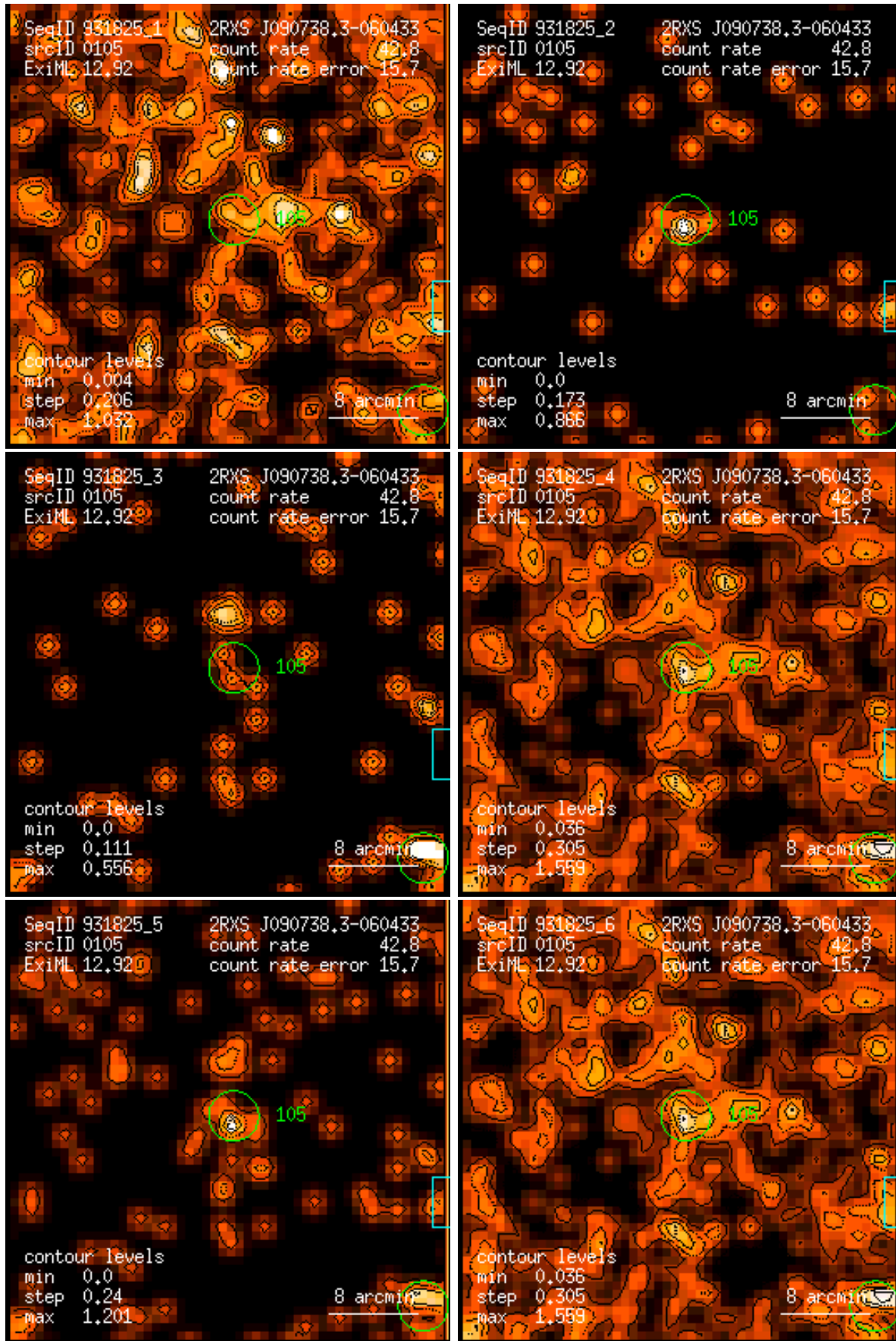
Figure 105: RASS 931825: detection 0105: band rate images, Gaussian filter: (1) PSPC channels 11 – 41, (2) 52 – 90, (3) 91 – 201, (4) 11 – 235, (5) 52 – 201, (6) 11 – 201. Broad band rates in counts/ks. Band rate contour levels in counts/ks/arcmin 2 .
