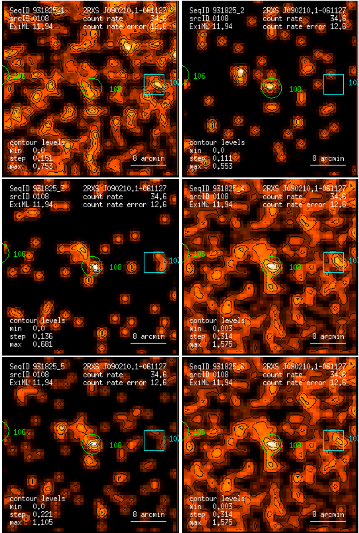
Figure 108: RASS 931825: detection 0108: band rate images, Gaussian filter: (1) PSPC channels 11 – 41, (2) 52 – 90, (3) 91 – 201, (4) 11 – 235, (5) 52 – 201, (6) 11 – 201. Broad band rates in counts/ks. Band rate contour levels in counts/ks/arcmin 2 .
