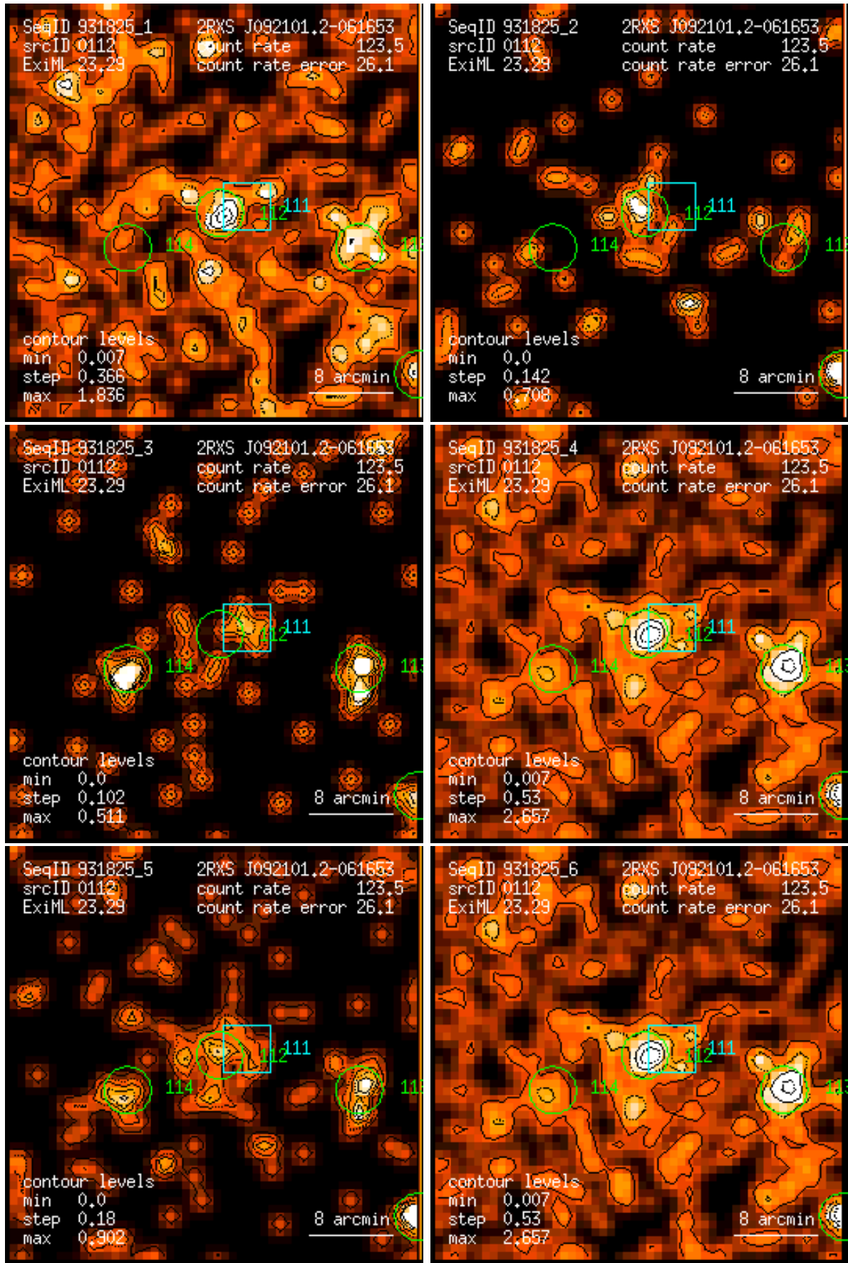
Figure 112: RASS 931825: detection 0112: band rate images, Gaussian filter: (1) PSPC channels 11 – 41, (2) 52 – 90, (3) 91 – 201, (4) 11 – 235, (5) 52 – 201, (6) 11 – 201. Broad band rates in counts/ks. Band rate contour levels in counts/ks/arcmin 2 .
