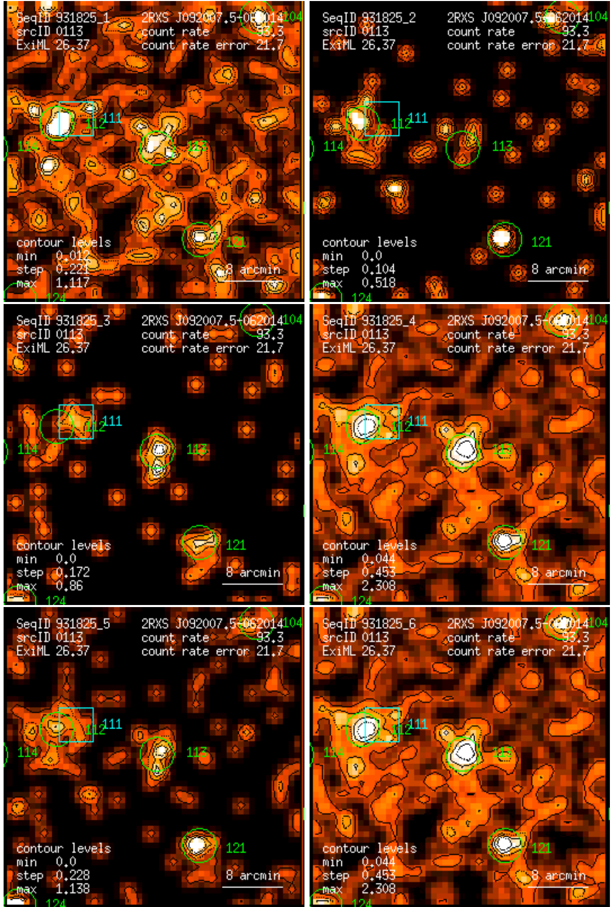
Figure 113: RASS 931825: detection 0113: band rate images, Gaussian filter: (1) PSPC channels 11 – 41, (2) 52 – 90, (3) 91 – 201, (4) 11 – 235, (5) 52 – 201, (6) 11 – 201. Broad band rates in counts/ks. Band rate contour levels in counts/ks/arcmin 2 .
