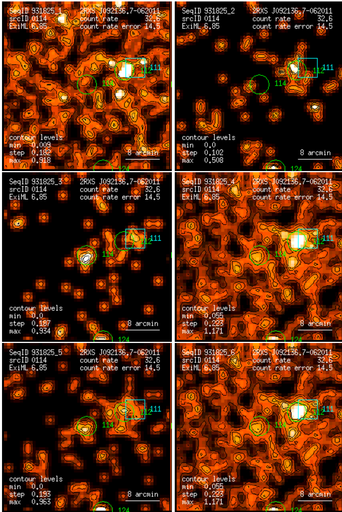
Figure 114: RASS 931825: detection 0114: band rate images, Gaussian filter: (1) PSPC channels 11 – 41, (2) 52 – 90, (3) 91 – 201, (4) 11 – 235, (5) 52 – 201, (6) 11 – 201. Broad band rates in counts/ks. Band rate contour levels in counts/ks/arcmin 2 .
