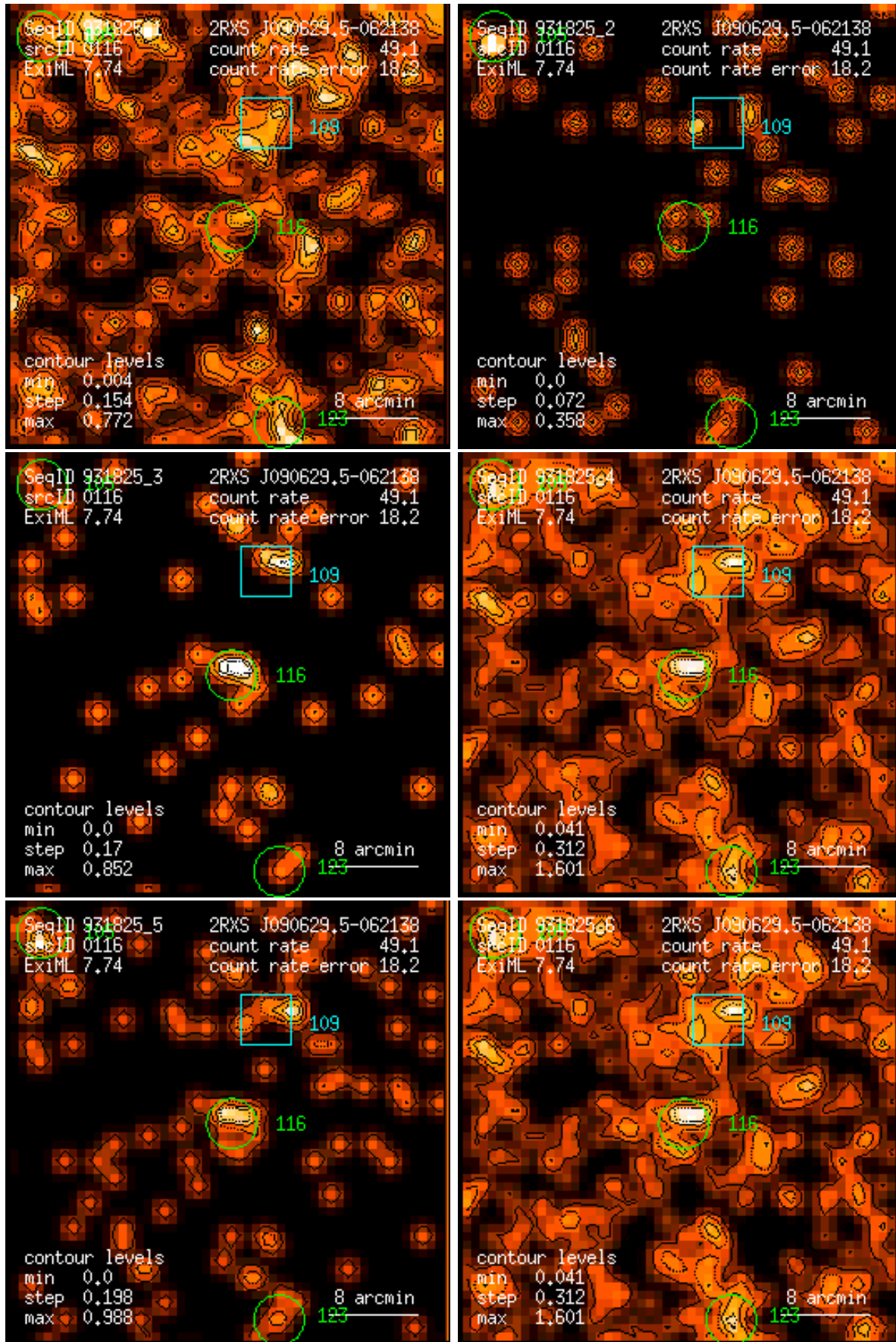
Figure 116: RASS 931825: detection 0116: band rate images, Gaussian filter: (1) PSPC channels 11 – 41, (2) 52 – 90, (3) 91 – 201, (4) 11 – 235, (5) 52 – 201, (6) 11 – 201. Broad band rates in counts/ks. Band rate contour levels in counts/ks/arcmin 2 .
