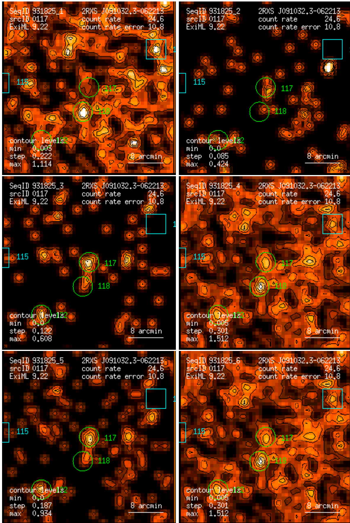
Figure 117: RASS 931825: detection 0117: band rate images, Gaussian filter: (1) PSPC channels 11 – 41, (2) 52 – 90, (3) 91 – 201, (4) 11 – 235, (5) 52 – 201, (6) 11 – 201. Broad band rates in counts/ks. Band rate contour levels in counts/ks/arcmin 2 .
