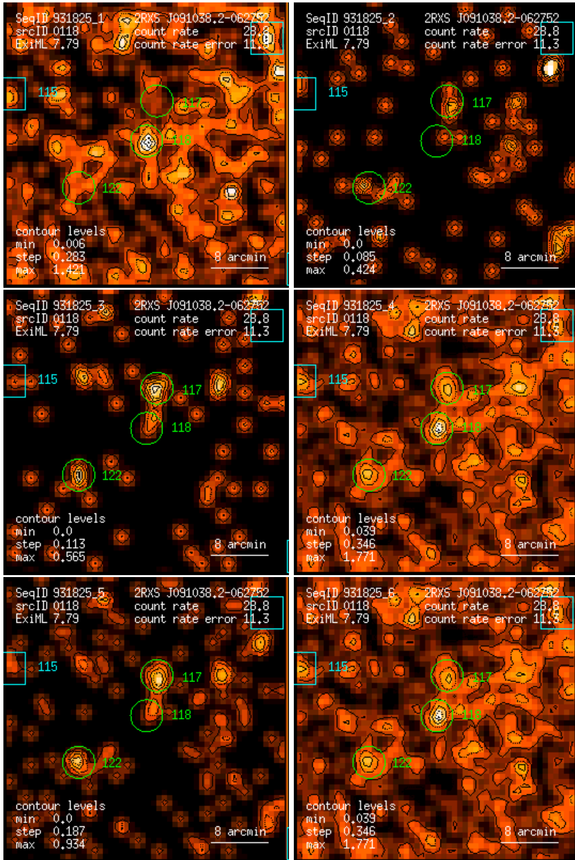
Figure 118: RASS 931825: detection 0118: band rate images, Gaussian filter: (1) PSPC channels 11 – 41, (2) 52 – 90, (3) 91 – 201, (4) 11 – 235, (5) 52 – 201, (6) 11 – 201. Broad band rates in counts/ks. Band rate contour levels in counts/ks/arcmin 2 .
