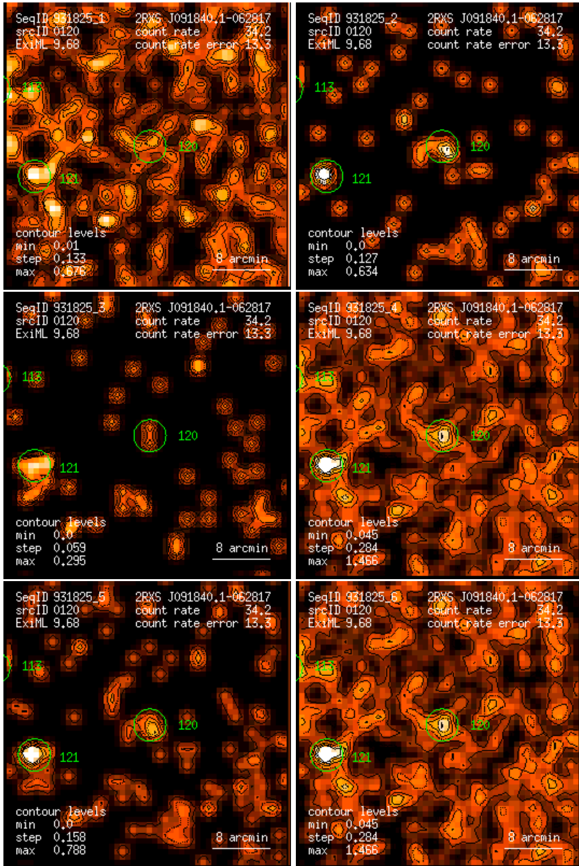
Figure 120: RASS 931825: detection 0120: band rate images, Gaussian filter: (1) PSPC channels 11 – 41, (2) 52 – 90, (3) 91 – 201, (4) 11 – 235, (5) 52 – 201, (6) 11 – 201. Broad band rates in counts/ks. Band rate contour levels in counts/ks/arcmin 2 .
