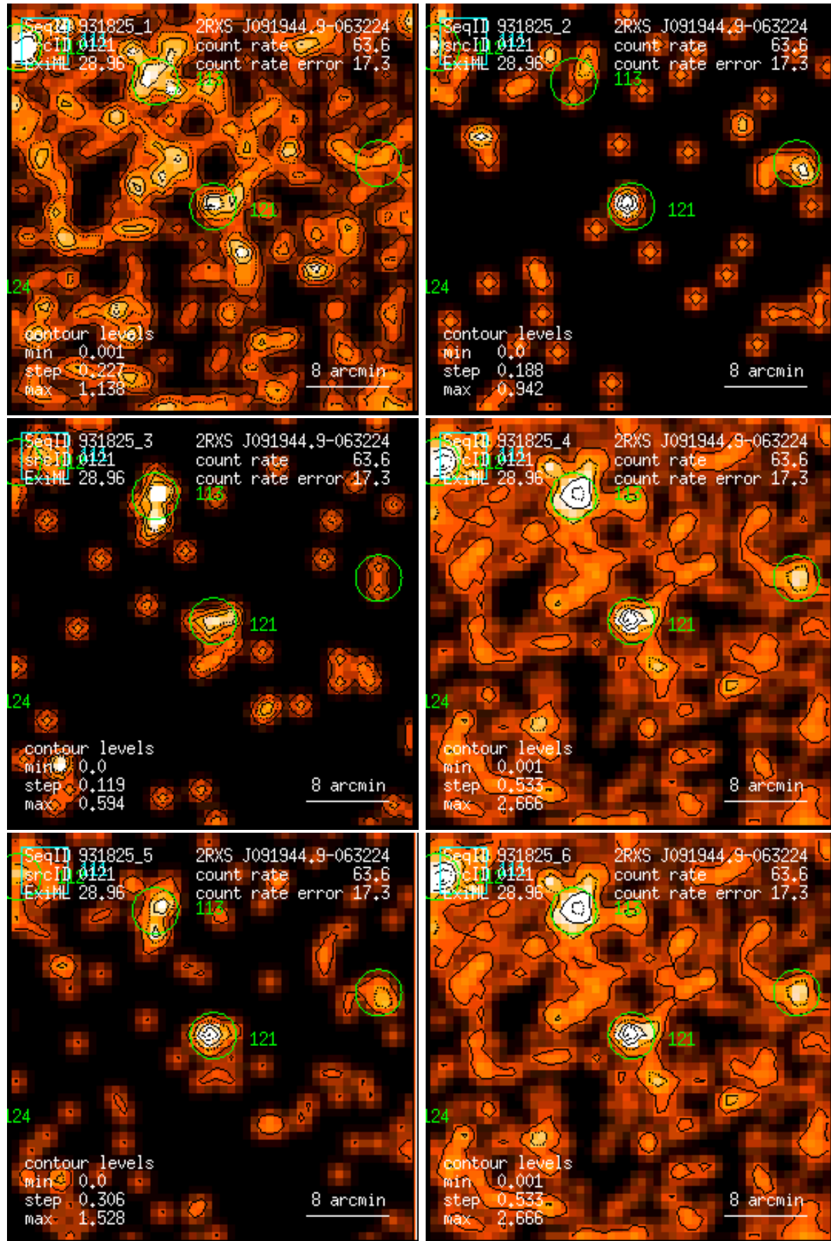
Figure 121: RASS 931825: detection 0121: band rate images, Gaussian filter: (1) PSPC channels 11 – 41, (2) 52 – 90, (3) 91 – 201, (4) 11 – 235, (5) 52 – 201, (6) 11 – 201. Broad band rates in counts/ks. Band rate contour levels in counts/ks/arcmin 2 .
