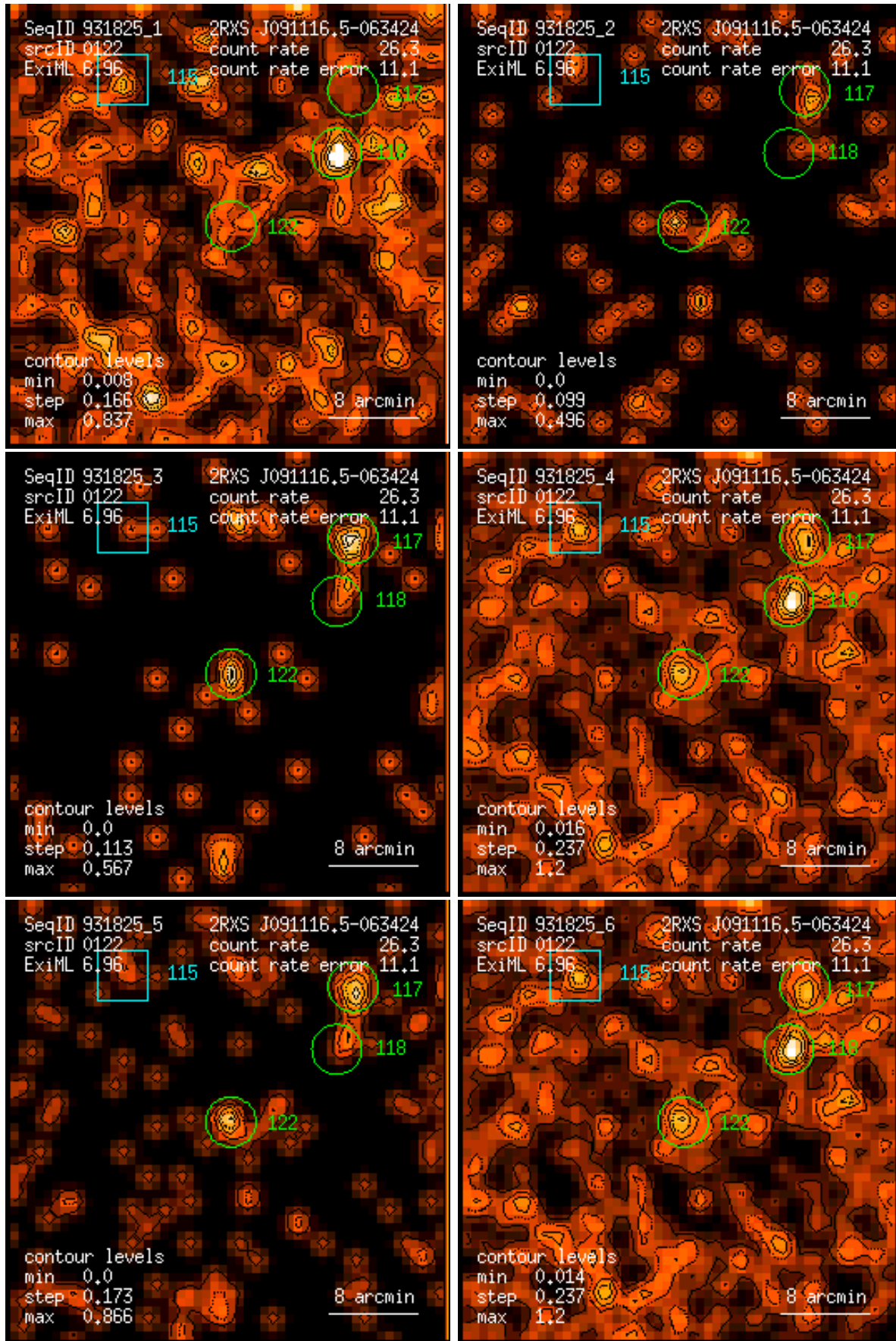
Figure 122: RASS 931825: detection 0122: band rate images, Gaussian filter: (1) PSPC channels 11 – 41, (2) 52 – 90, (3) 91 – 201, (4) 11 – 235, (5) 52 – 201, (6) 11 – 201. Broad band rates in counts/ks. Band rate contour levels in counts/ks/arcmin 2 .
