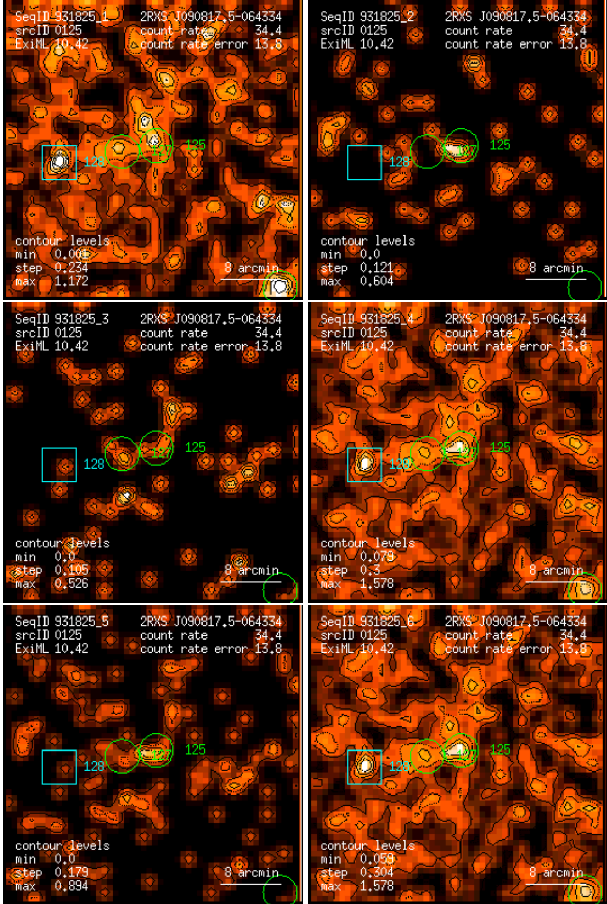
Figure 125: RASS 931825: detection 0125: band rate images, Gaussian filter: (1) PSPC channels 11 – 41, (2) 52 – 90, (3) 91 – 201, (4) 11 – 235, (5) 52 – 201, (6) 11 – 201. Broad band rates in counts/ks. Band rate contour levels in counts/ks/arcmin 2 .
