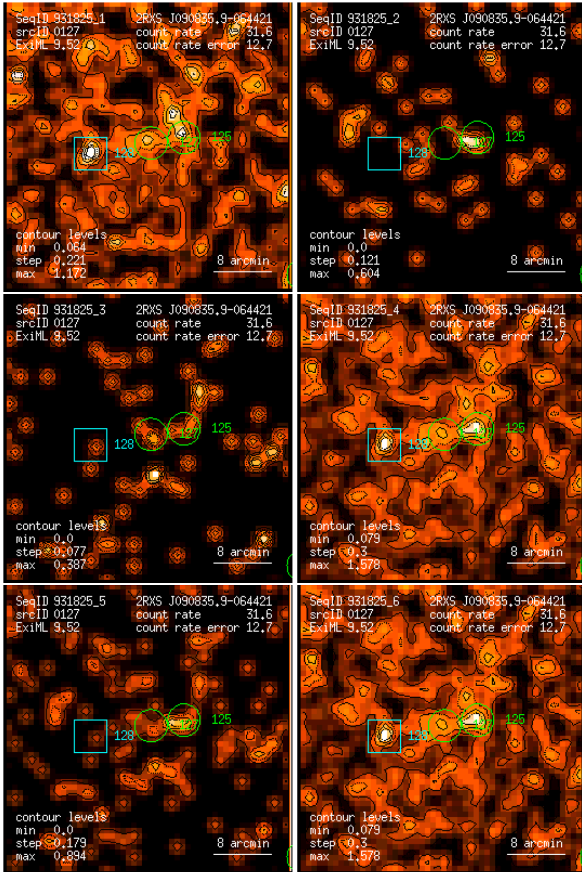
Figure 127: RASS 931825: detection 0127: band rate images, Gaussian filter: (1) PSPC channels 11 – 41, (2) 52 – 90, (3) 91 – 201, (4) 11 – 235, (5) 52 – 201, (6) 11 – 201. Broad band rates in counts/ks. Band rate contour levels in counts/ks/arcmin 2 .
