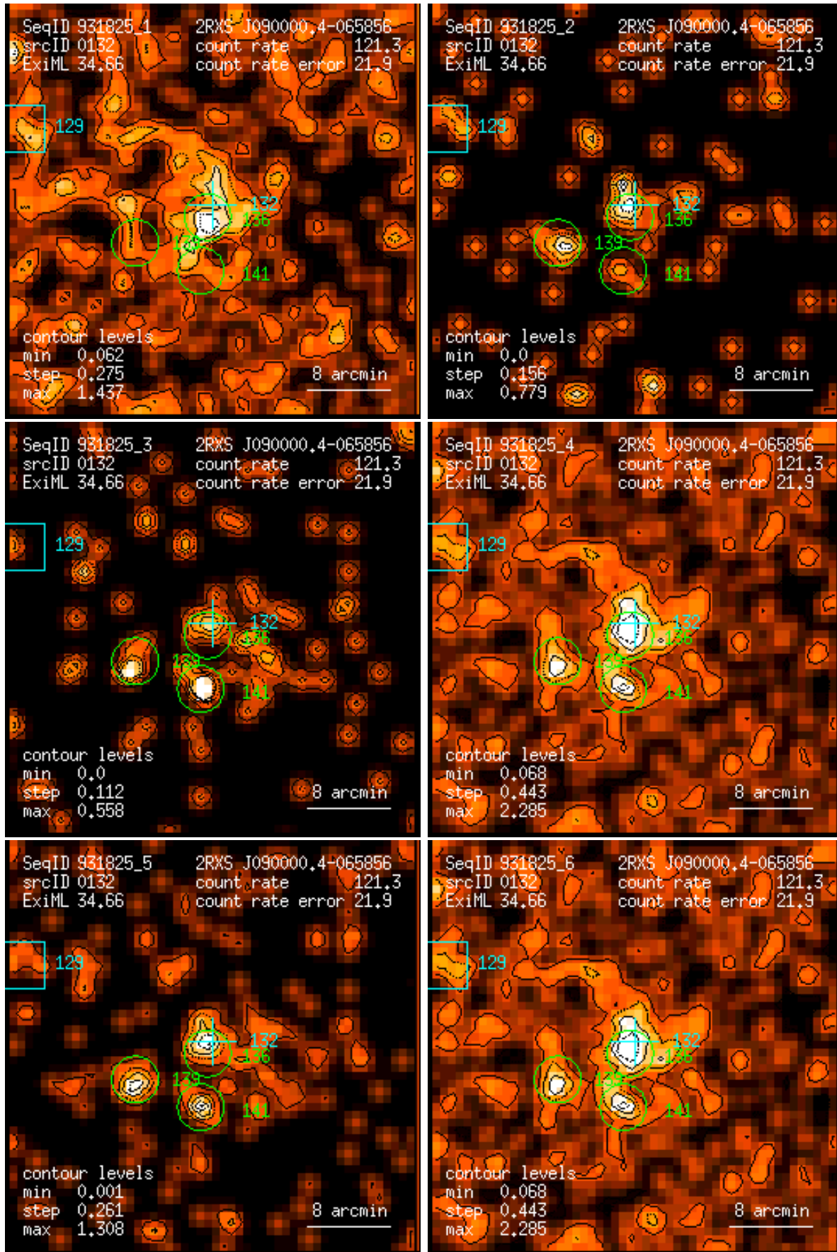
Figure 132: RASS 931825: detection 0132: band rate images, Gaussian filter: (1) PSPC channels 11 – 41, (2) 52 – 90, (3) 91 – 201, (4) 11 – 235, (5) 52 – 201, (6) 11 – 201. Broad band rates in counts/ks. Band rate contour levels in counts/ks/arcmin 2 .
