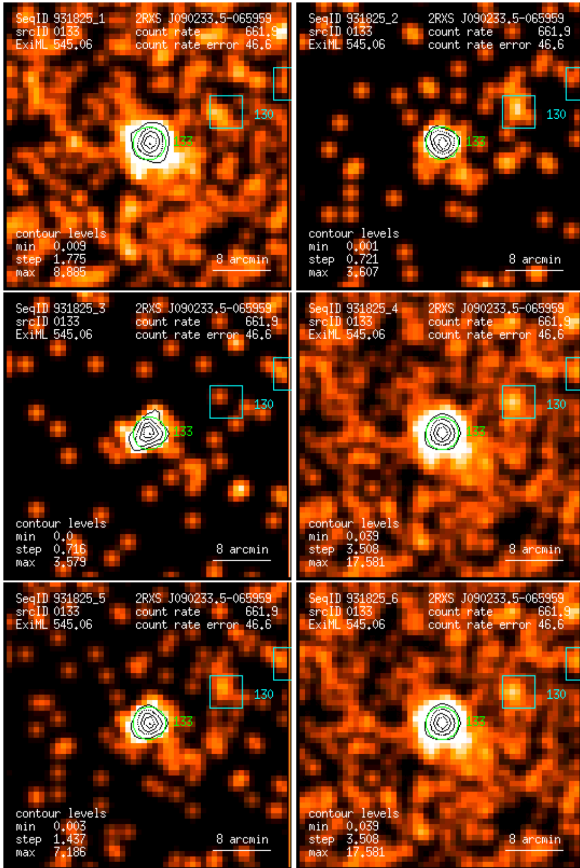
Figure 133: RASS 931825: detection 0133: band rate images, Gaussian filter: (1) PSPC channels 11 – 41, (2) 52 – 90, (3) 91 – 201, (4) 11 – 235, (5) 52 – 201, (6) 11 – 201. Broad band rates in counts/ks. Band rate contour levels in counts/ks/arcmin 2 .
