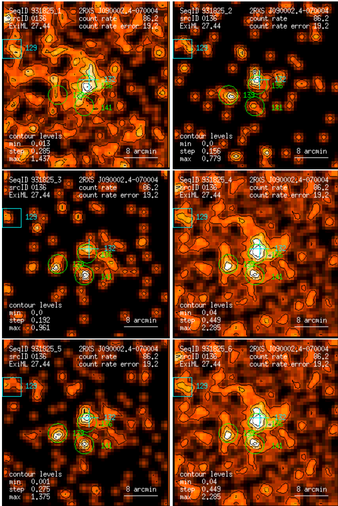
Figure 136: RASS 931825: detection 0136: band rate images, Gaussian filter: (1) PSPC channels 11 – 41, (2) 52 – 90, (3) 91 – 201, (4) 11 – 235, (5) 52 – 201, (6) 11 – 201. Broad band rates in counts/ks. Band rate contour levels in counts/ks/arcmin 2 .
