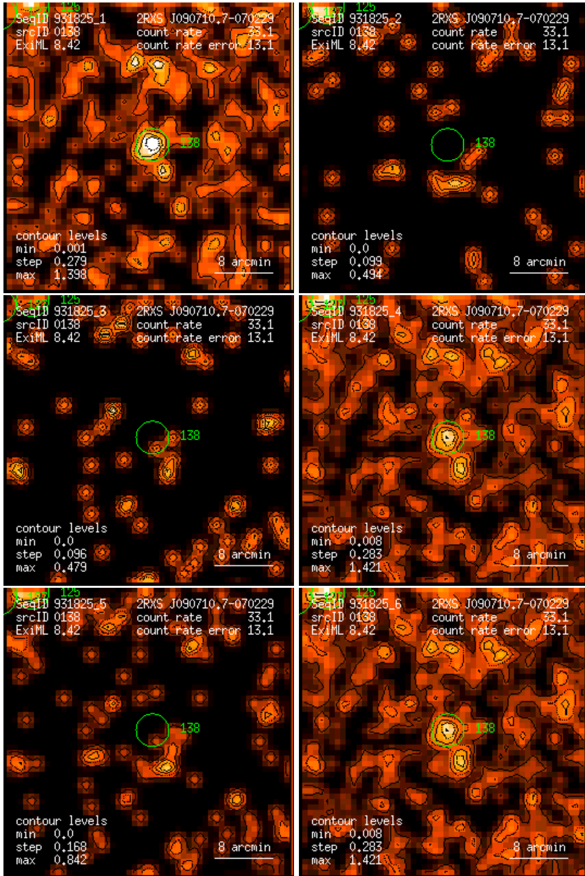
Figure 138: RASS 931825: detection 0138: band rate images, Gaussian filter: (1) PSPC channels 11 – 41, (2) 52 – 90, (3) 91 – 201, (4) 11 – 235, (5) 52 – 201, (6) 11 – 201. Broad band rates in counts/ks. Band rate contour levels in counts/ks/arcmin 2 .
