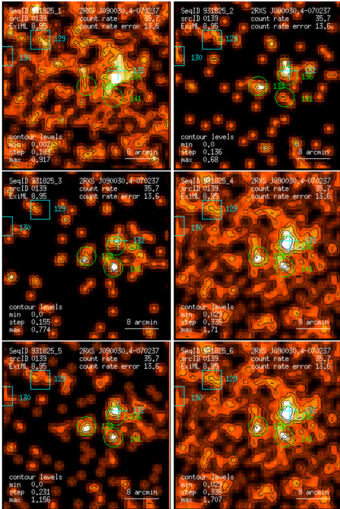
Figure 139: RASS 931825: detection 0139: band rate images, Gaussian filter: (1) PSPC channels 11 – 41, (2) 52 – 90, (3) 91 – 201, (4) 11 – 235, (5) 52 – 201, (6) 11 – 201. Broad band rates in counts/ks. Band rate contour levels in counts/ks/arcmin 2 .
