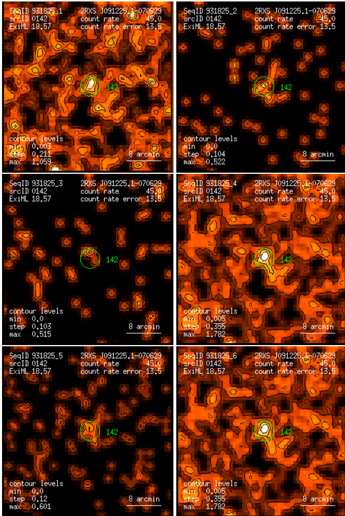
Figure 142: RASS 931825: detection 0142: band rate images, Gaussian filter: (1) PSPC channels 11 – 41, (2) 52 – 90, (3) 91 – 201, (4) 11 – 235, (5) 52 – 201, (6) 11 – 201. Broad band rates in counts/ks. Band rate contour levels in counts/ks/arcmin 2 .
