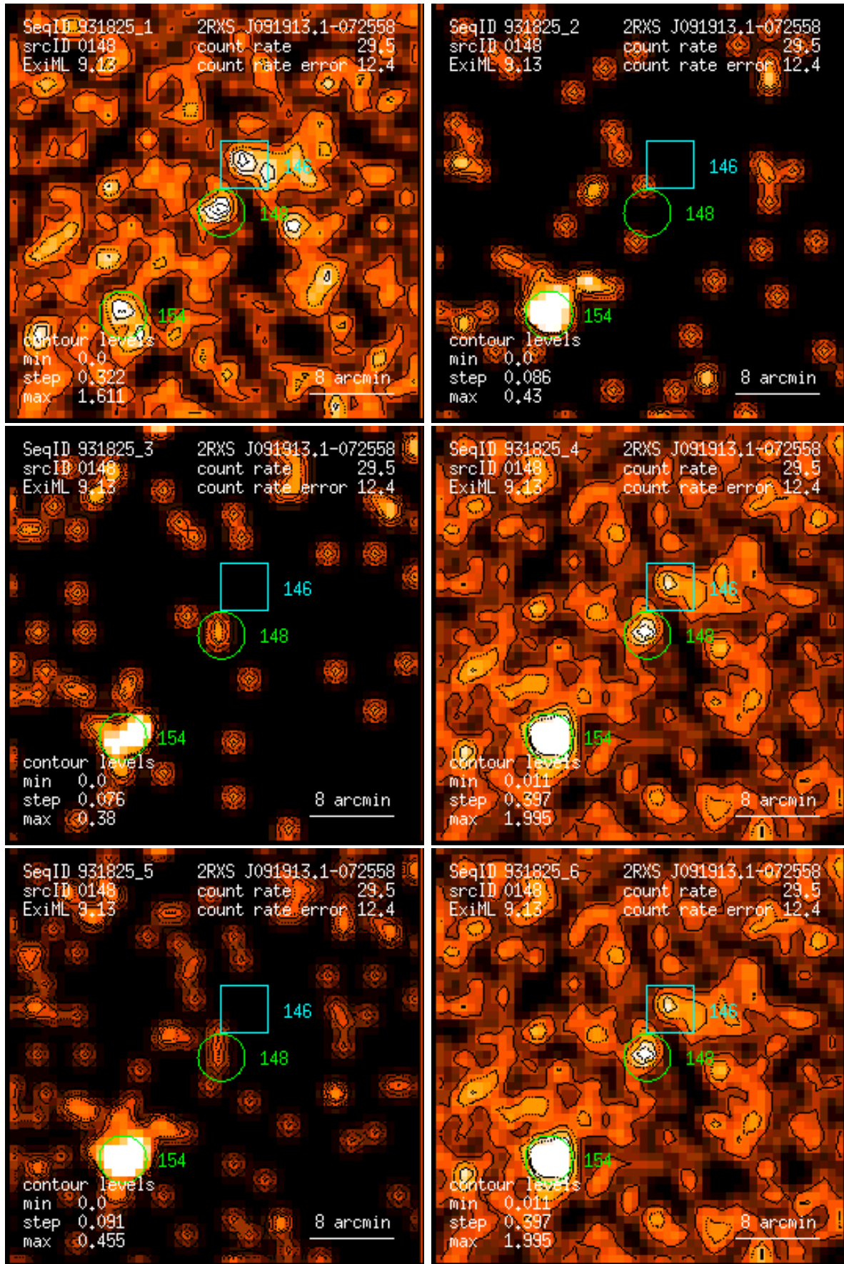
Figure 148: RASS 931825: detection 0148: band rate images, Gaussian filter: (1) PSPC channels 11 – 41, (2) 52 – 90, (3) 91 – 201, (4) 11 – 235, (5) 52 – 201, (6) 11 – 201. Broad band rates in counts/ks. Band rate contour levels in counts/ks/arcmin 2 .
