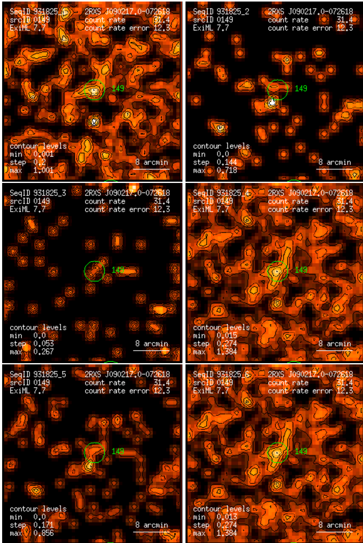
Figure 149: RASS 931825: detection 0149: band rate images, Gaussian filter: (1) PSPC channels 11 – 41, (2) 52 – 90, (3) 91 – 201, (4) 11 – 235, (5) 52 – 201, (6) 11 – 201. Broad band rates in counts/ks. Band rate contour levels in counts/ks/arcmin 2 .
