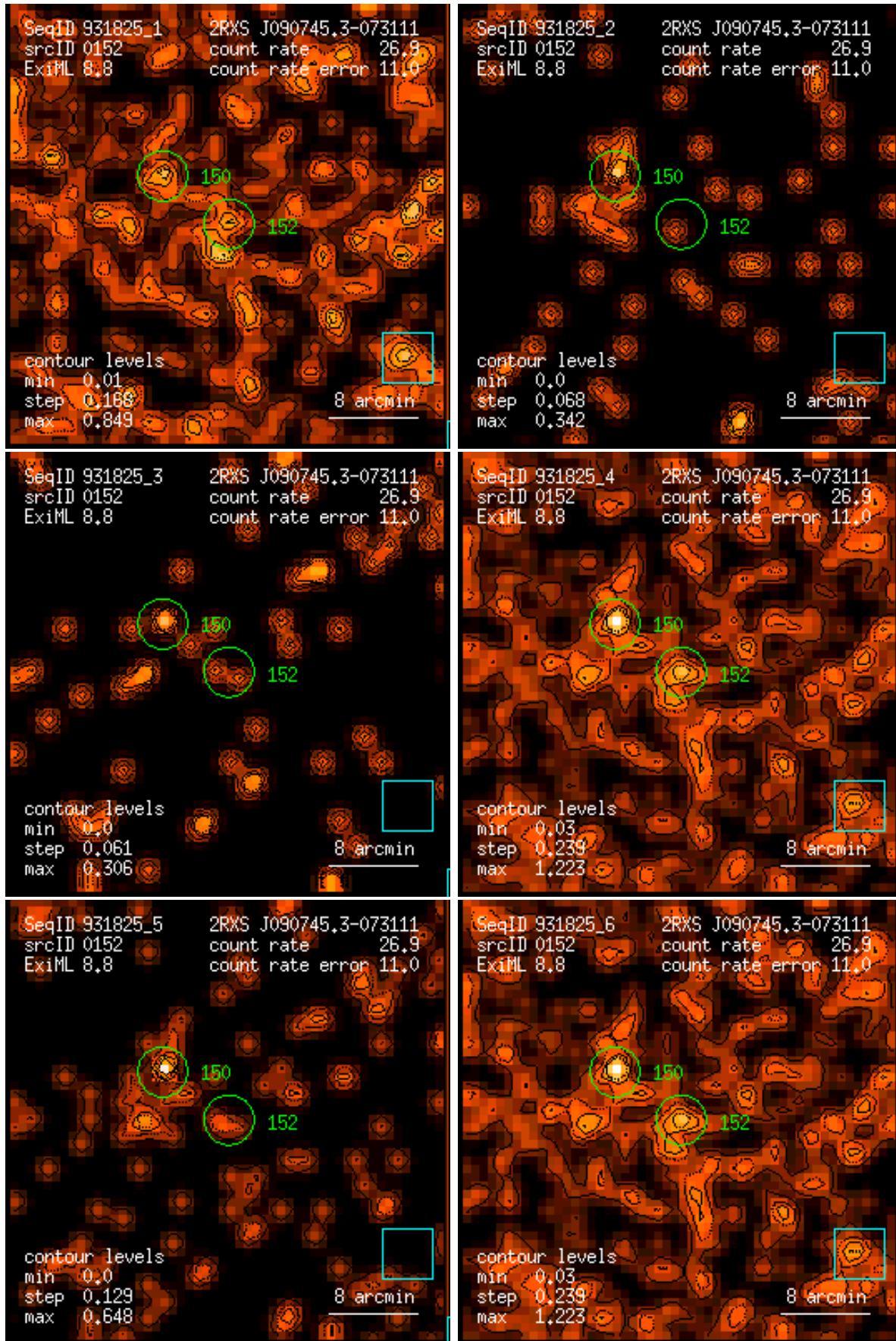
Figure 152: RASS 931825: detection 0152: band rate images, Gaussian filter: (1) PSPC channels 11 – 41, (2) 52 – 90, (3) 91 – 201, (4) 11 – 235, (5) 52 – 201, (6) 11 – 201. Broad band rates in counts/ks. Band rate contour levels in counts/ks/arcmin 2 .
