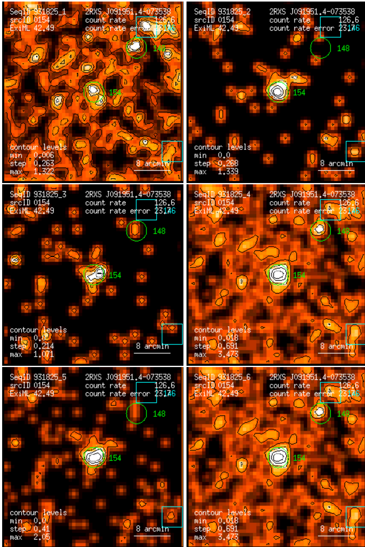
Figure 154: RASS 931825: detection 0154: band rate images, Gaussian filter: (1) PSPC channels 11 – 41, (2) 52 – 90, (3) 91 – 201, (4) 11 – 235, (5) 52 – 201, (6) 11 – 201. Broad band rates in counts/ks. Band rate contour levels in counts/ks/arcmin 2 .
