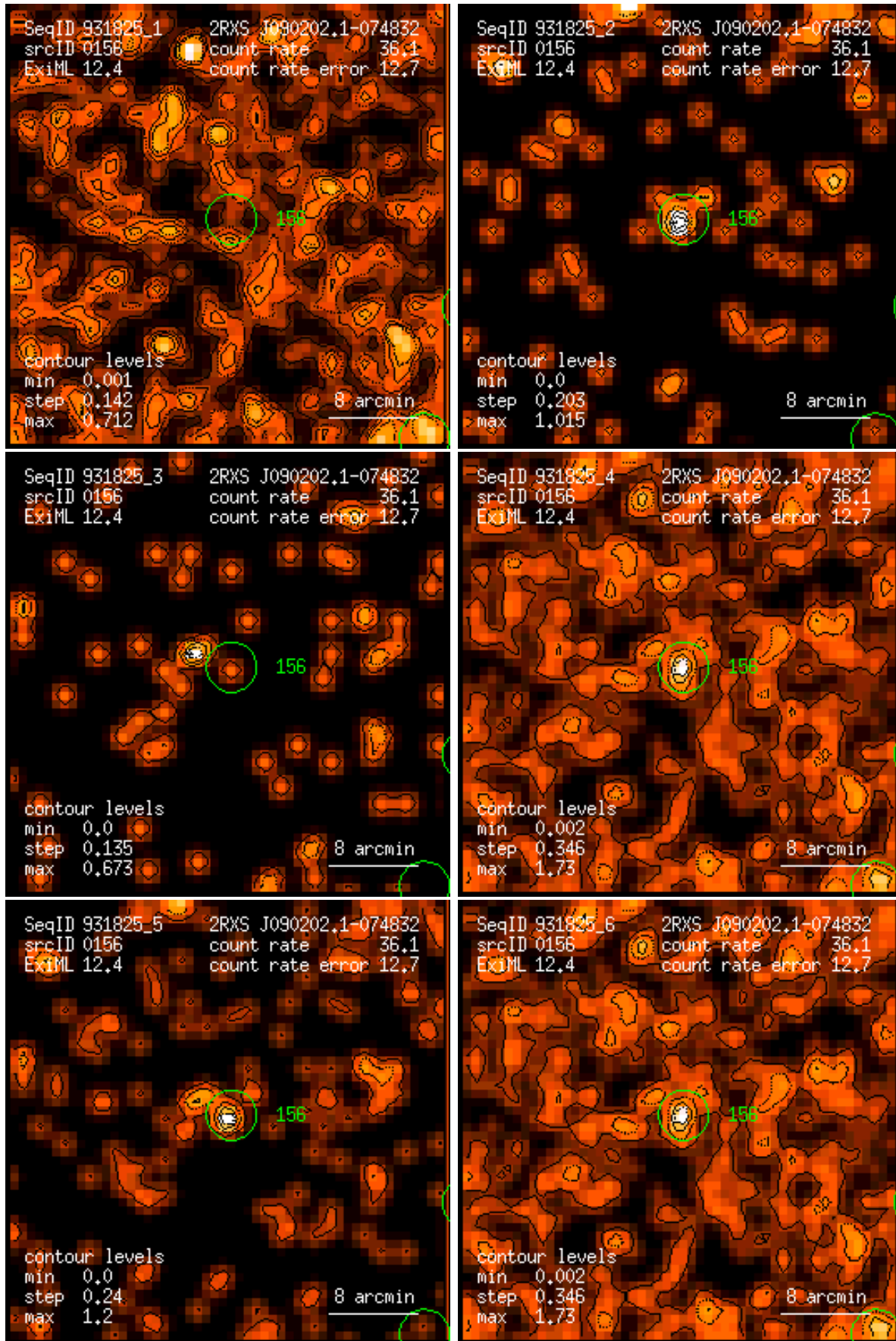
Figure 156: RASS 931825: detection 0156: band rate images, Gaussian filter: (1) PSPC channels 11 – 41, (2) 52 – 90, (3) 91 – 201, (4) 11 – 235, (5) 52 – 201, (6) 11 – 201. Broad band rates in counts/ks. Band rate contour levels in counts/ks/arcmin 2 .
