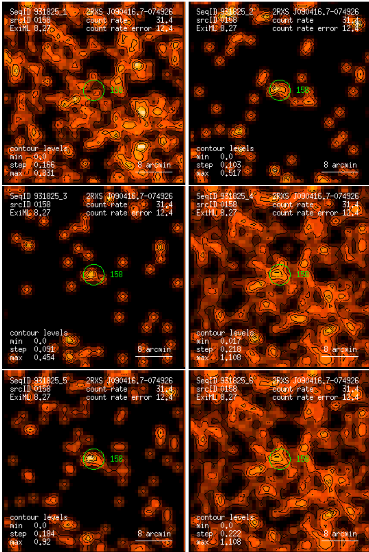
Figure 158: RASS 931825: detection 0158: band rate images, Gaussian filter: (1) PSPC channels 11 – 41, (2) 52 – 90, (3) 91 – 201, (4) 11 – 235, (5) 52 – 201, (6) 11 – 201. Broad band rates in counts/ks. Band rate contour levels in counts/ks/arcmin 2 .
