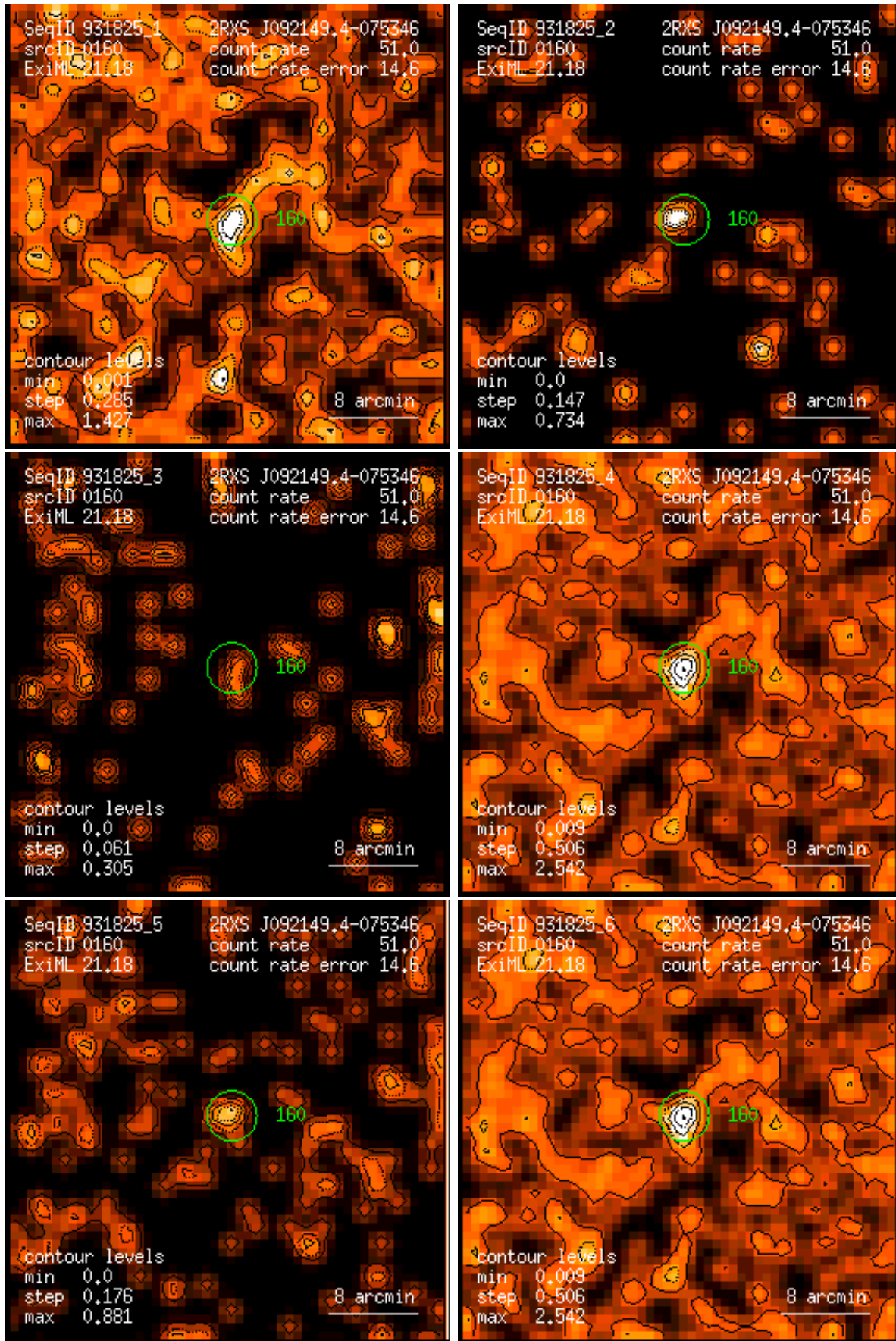
Figure 160: RASS 931825: detection 0160: band rate images, Gaussian filter: (1) PSPC channels 11 – 41, (2) 52 – 90, (3) 91 – 201, (4) 11 – 235, (5) 52 – 201, (6) 11 – 201. Broad band rates in counts/ks. Band rate contour levels in counts/ks/arcmin 2 .
