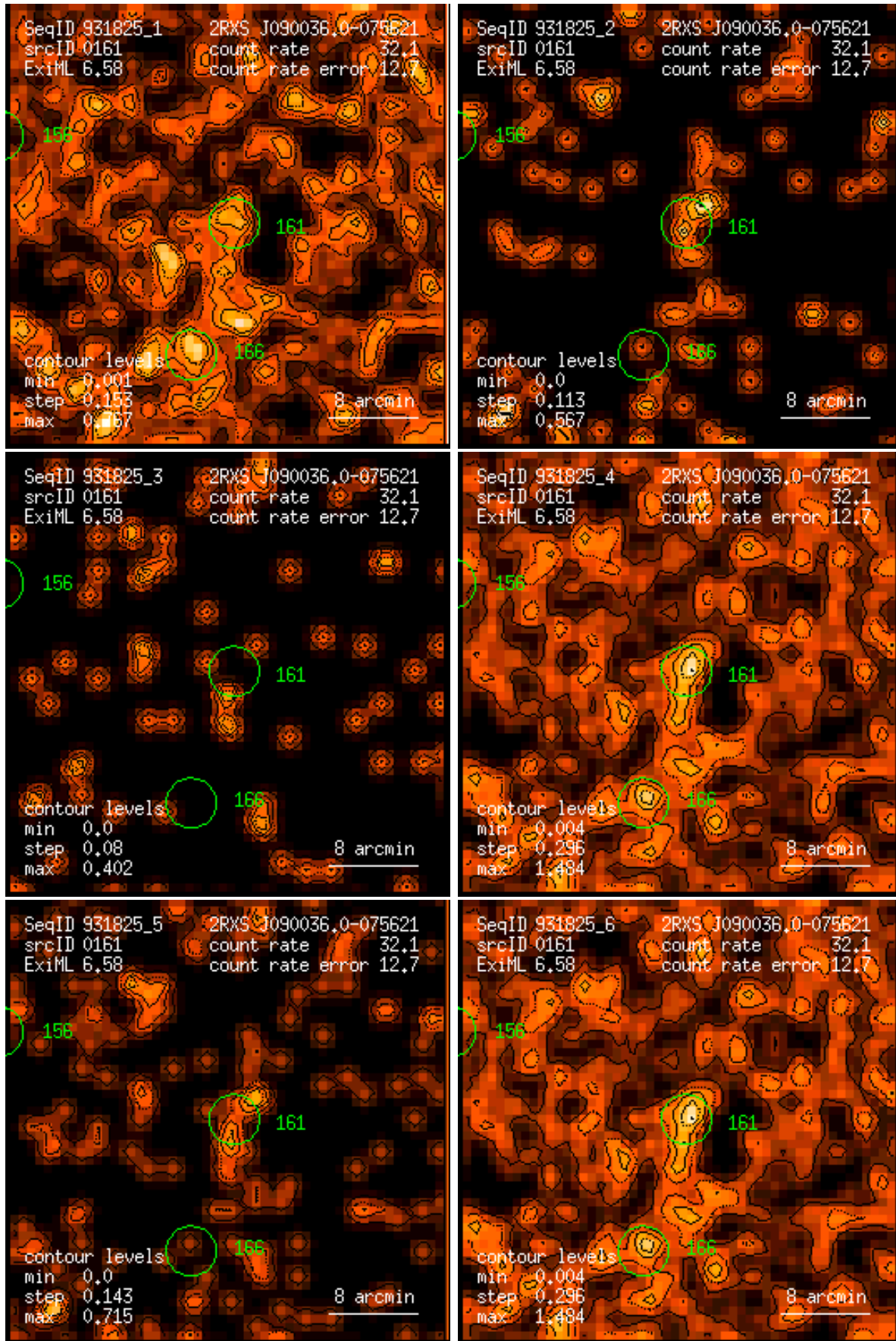
Figure 161: RASS 931825: detection 0161: band rate images, Gaussian filter: (1) PSPC channels 11 – 41, (2) 52 – 90, (3) 91 – 201, (4) 11 – 235, (5) 52 – 201, (6) 11 – 201. Broad band rates in counts/ks. Band rate contour levels in counts/ks/arcmin 2 .
