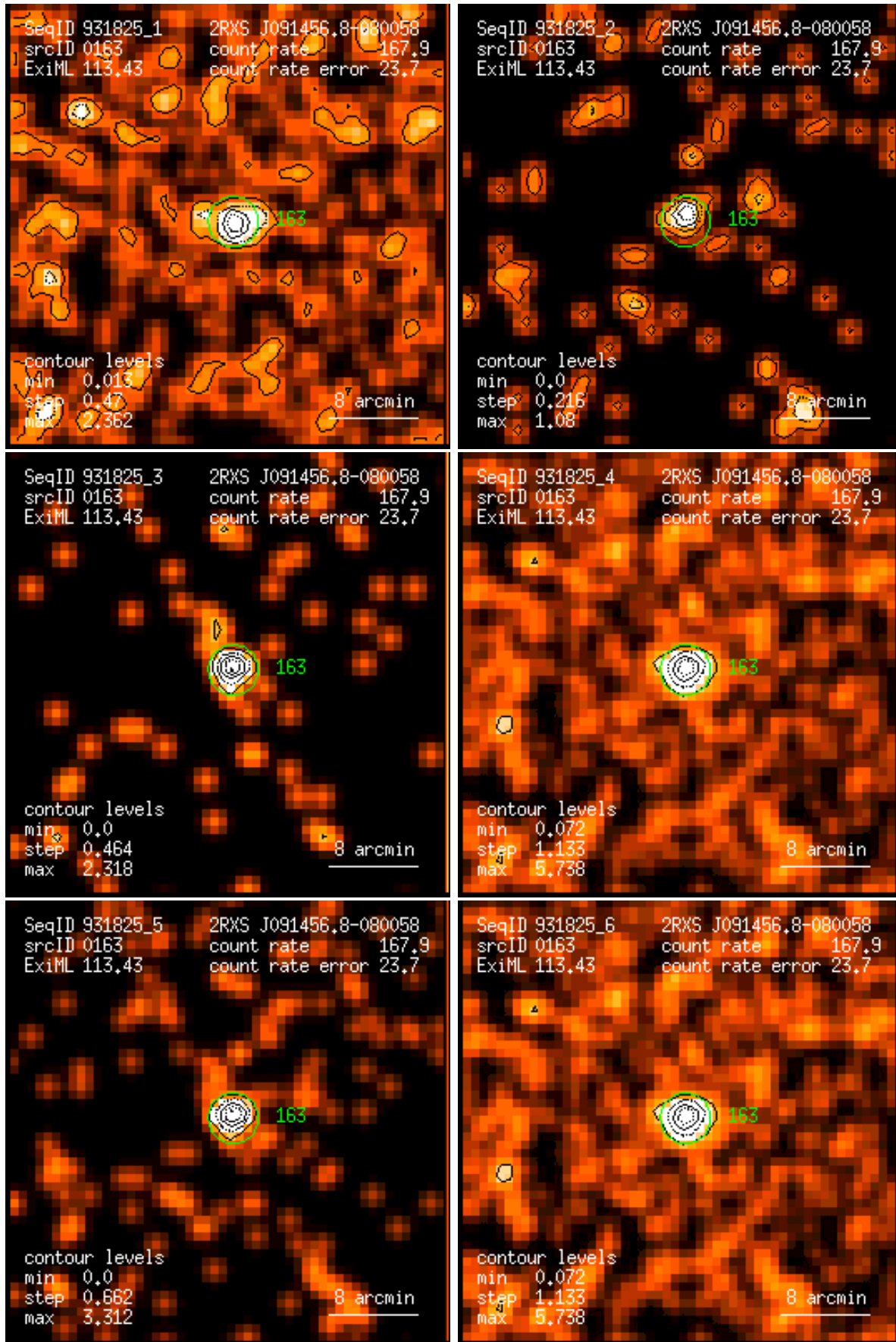
Figure 163: RASS 931825: detection 0163: band rate images, Gaussian filter: (1) PSPC channels 11 – 41, (2) 52 – 90, (3) 91 – 201, (4) 11 – 235, (5) 52 – 201, (6) 11 – 201. Broad band rates in counts/ks. Band rate contour levels in counts/ks/arcmin 2 .
