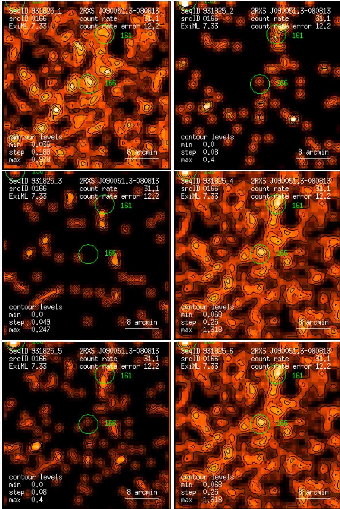
Figure 166: RASS 931825: detection 0166: band rate images, Gaussian filter: (1) PSPC channels 11 – 41, (2) 52 – 90, (3) 91 – 201, (4) 11 – 235, (5) 52 – 201, (6) 11 – 201. Broad band rates in counts/ks. Band rate contour levels in counts/ks/arcmin 2 .
