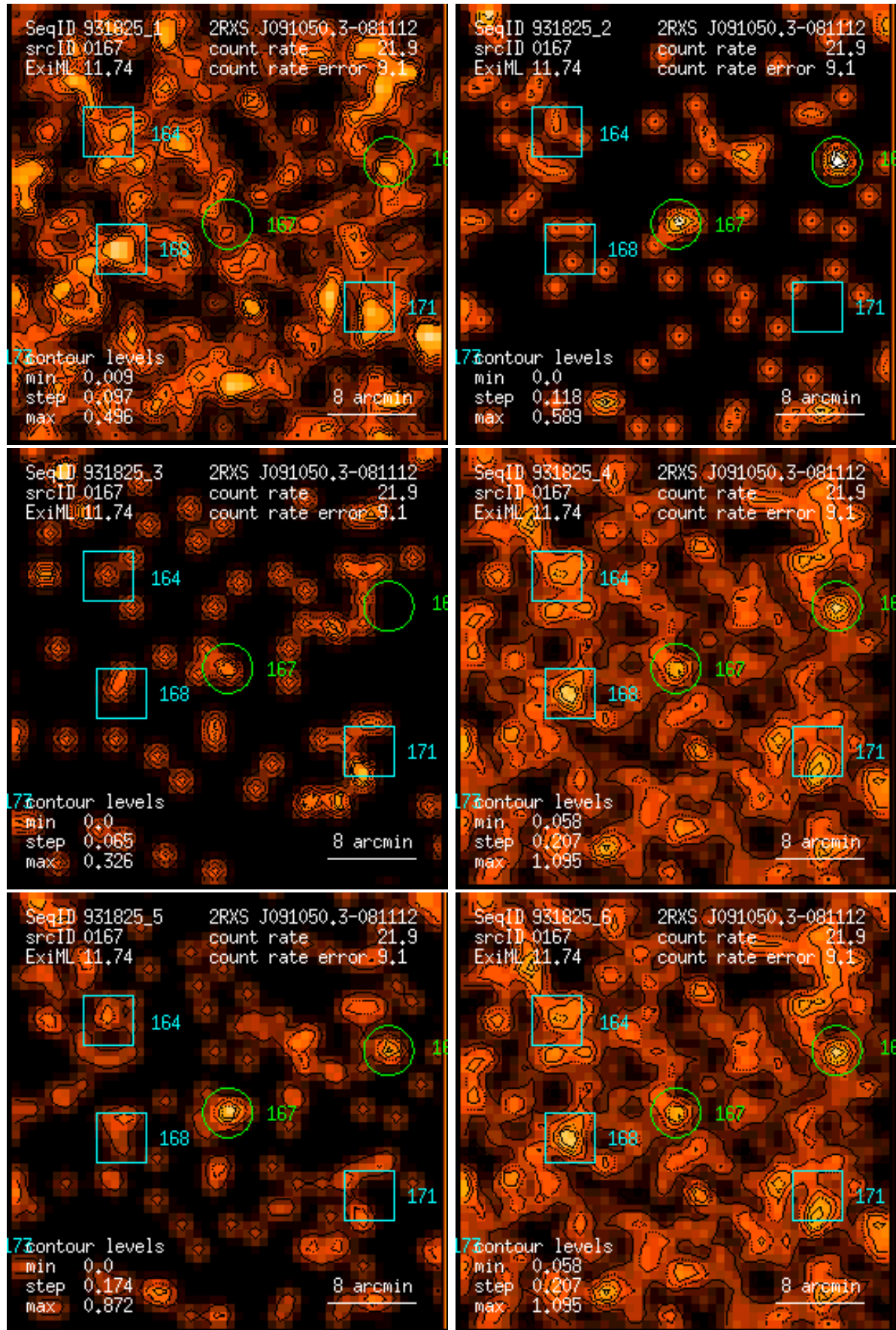
Figure 167: RASS 931825: detection 0167: band rate images, Gaussian filter: (1) PSPC channels 11 – 41, (2) 52 – 90, (3) 91 – 201, (4) 11 – 235, (5) 52 – 201, (6) 11 – 201. Broad band rates in counts/ks. Band rate contour levels in counts/ks/arcmin 2 .
