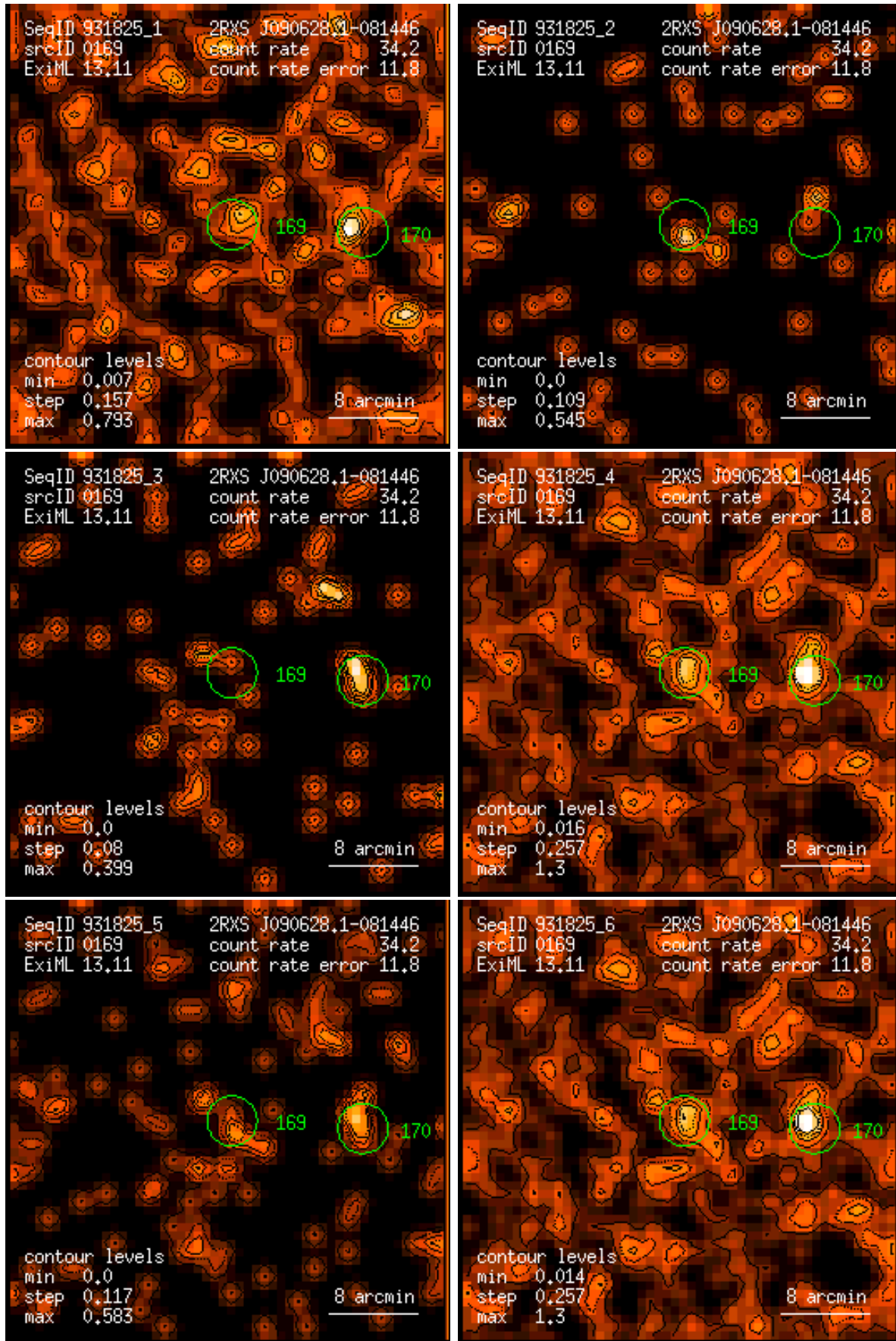
Figure 169: RASS 931825: detection 0169: band rate images, Gaussian filter: (1) PSPC channels 11 – 41, (2) 52 – 90, (3) 91 – 201, (4) 11 – 235, (5) 52 – 201, (6) 11 – 201. Broad band rates in counts/ks. Band rate contour levels in counts/ks/arcmin 2 .
