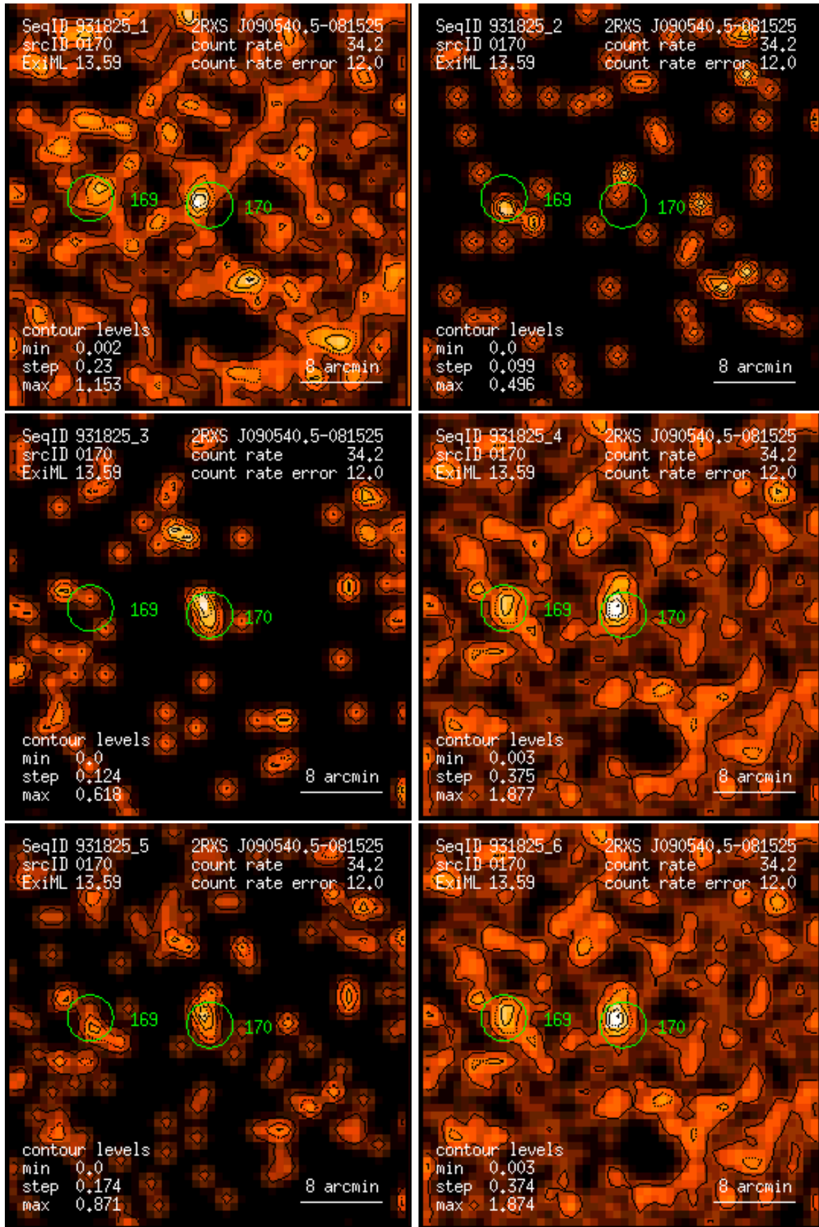
Figure 170: RASS 931825: detection 0170: band rate images, Gaussian filter: (1) PSPC channels 11 – 41, (2) 52 – 90, (3) 91 – 201, (4) 11 – 235, (5) 52 – 201, (6) 11 – 201. Broad band rates in counts/ks. Band rate contour levels in counts/ks/arcmin 2 .
