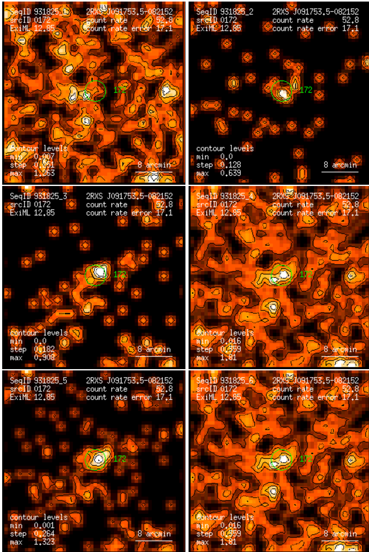
Figure 172: RASS 931825: detection 0172: band rate images, Gaussian filter: (1) PSPC channels 11 – 41, (2) 52 – 90, (3) 91 – 201, (4) 11 – 235, (5) 52 – 201, (6) 11 – 201. Broad band rates in counts/ks. Band rate contour levels in counts/ks/arcmin 2 .
