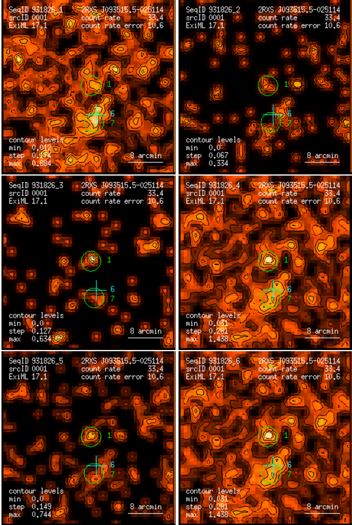
Figure 1: RASS 931826: detection 0001: band rate images, Gaussian filter: (1) PSPC channels 11 – 41, (2) 52 – 90, (3) 91 – 201, (4) 11 – 235, (5) 52 – 201, (6) 11 – 201. Broad band rates in counts/ks. Band rate contour levels in counts/ks/arcmin 2 .
