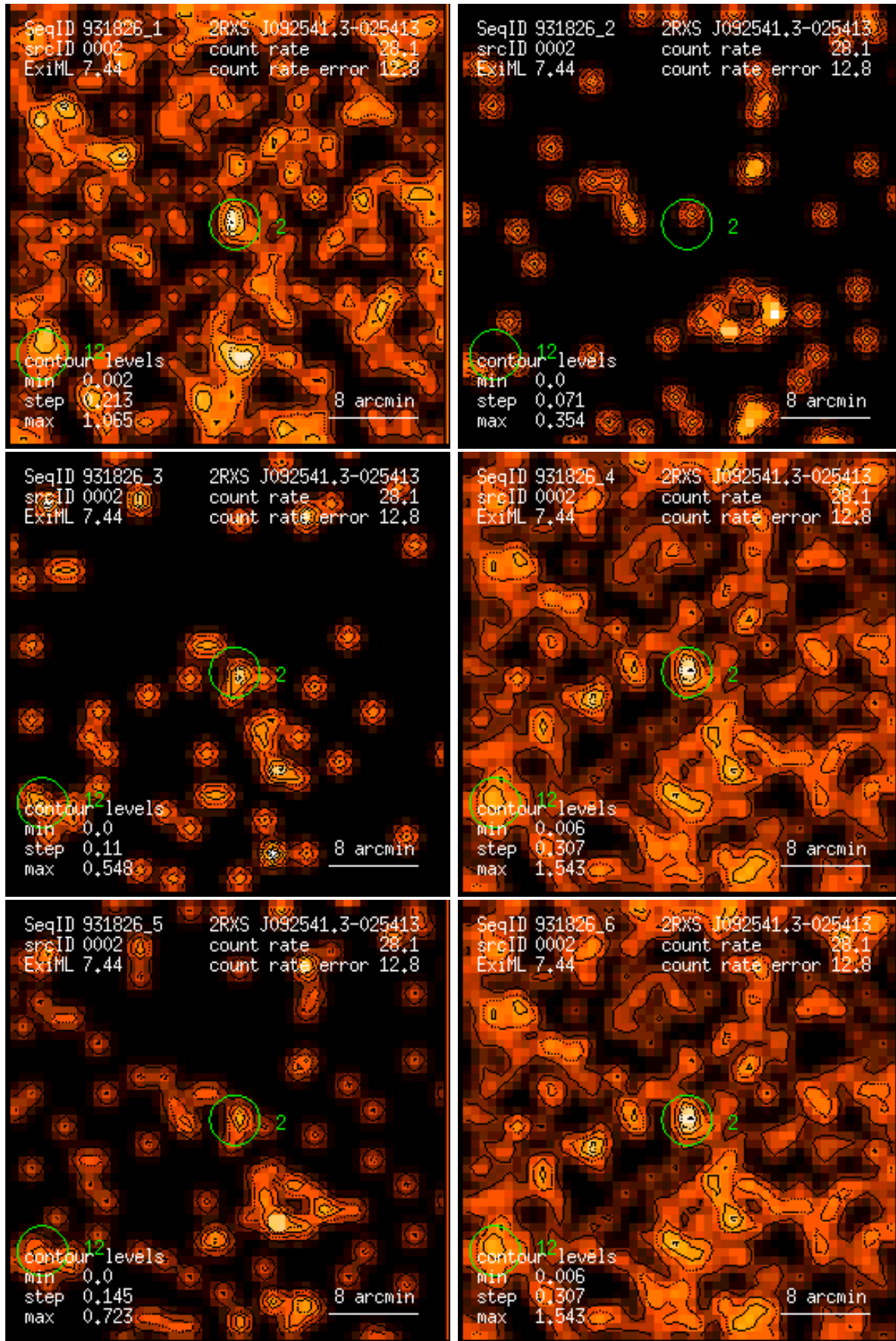
Figure 2: RASS 931826: detection 0002: band rate images, Gaussian filter: (1) PSPC channels 11 – 41, (2) 52 – 90, (3) 91 – 201, (4) 11 – 235, (5) 52 – 201, (6) 11 – 201. Broad band rates in counts/ks. Band rate contour levels in counts/ks/arcmin 2 .
