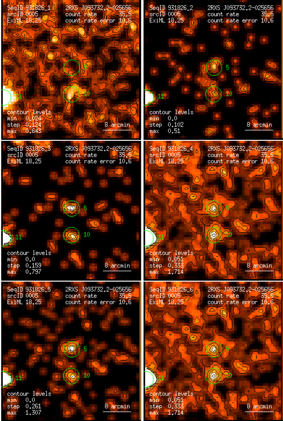
Figure 5: RASS 931826: detection 0005: band rate images, Gaussian filter: (1) PSPC channels 11 – 41, (2) 52 – 90, (3) 91 – 201, (4) 11 – 235, (5) 52 – 201, (6) 11 – 201. Broad band rates in counts/ks. Band rate contour levels in counts/ks/arcmin 2 .
