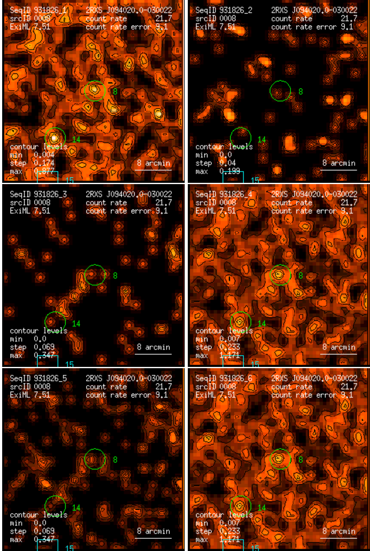
Figure 8: RASS 931826: detection 0008: band rate images, Gaussian filter: (1) PSPC channels 11 – 41, (2) 52 – 90, (3) 91 – 201, (4) 11 – 235, (5) 52 – 201, (6) 11 – 201. Broad band rates in counts/ks. Band rate contour levels in counts/ks/arcmin 2 .
