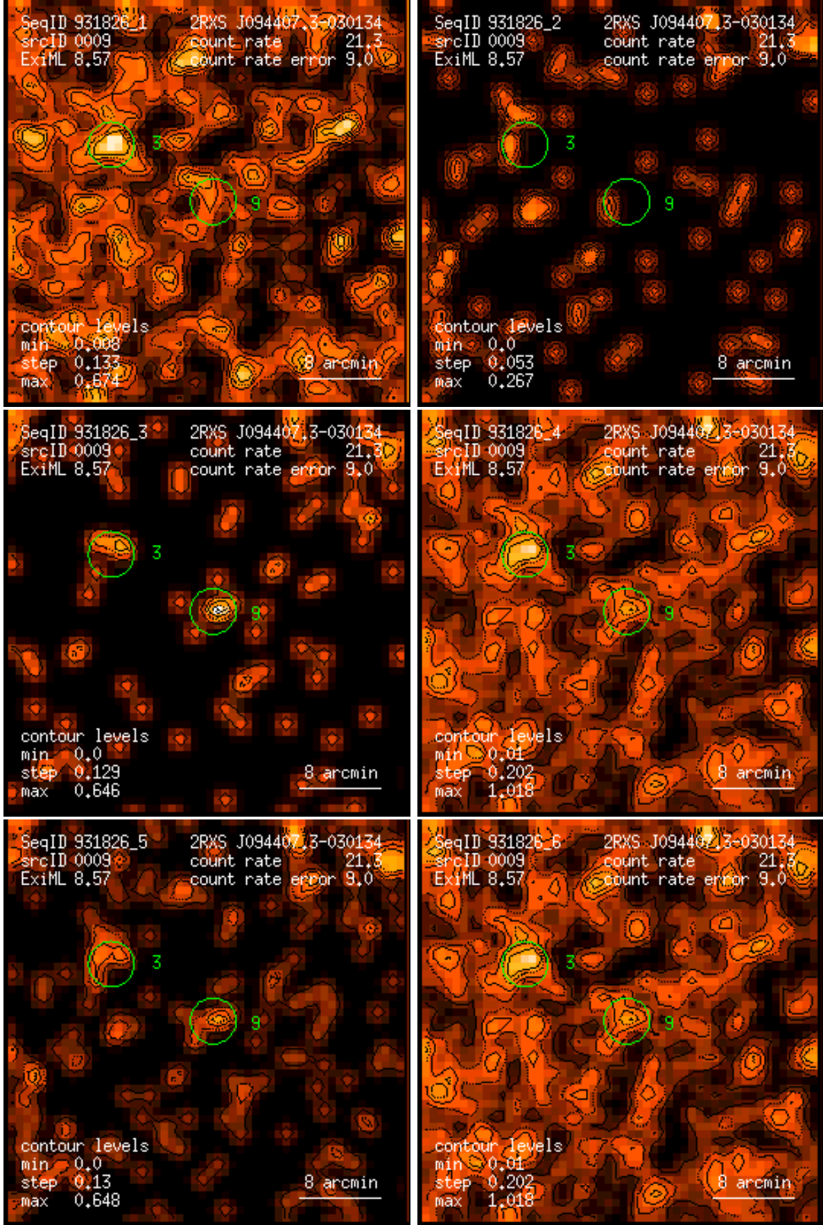
Figure 9: RASS 931826: detection 0009: band rate images, Gaussian filter: (1) PSPC channels 11 – 41, (2) 52 – 90, (3) 91 – 201, (4) 11 – 235, (5) 52 – 201, (6) 11 – 201. Broad band rates in counts/ks. Band rate contour levels in counts/ks/arcmin 2 .
