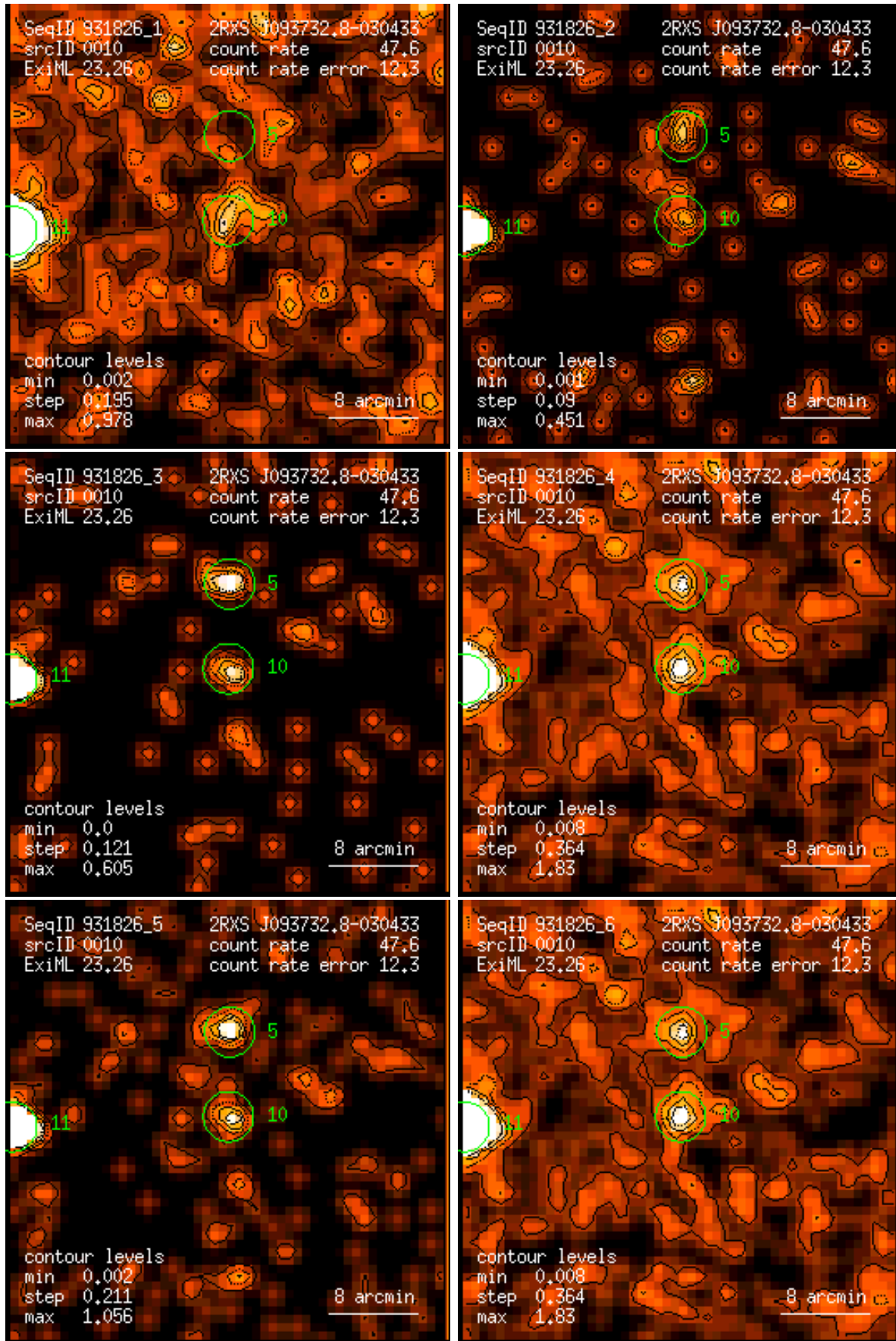
Figure 10: RASS 931826: detection 0010: band rate images, Gaussian filter: (1) PSPC channels 11 – 41, (2) 52 – 90, (3) 91 – 201, (4) 11 – 235, (5) 52 – 201, (6) 11 – 201. Broad band rates in counts/ks. Band rate contour levels in counts/ks/arcmin 2 .
