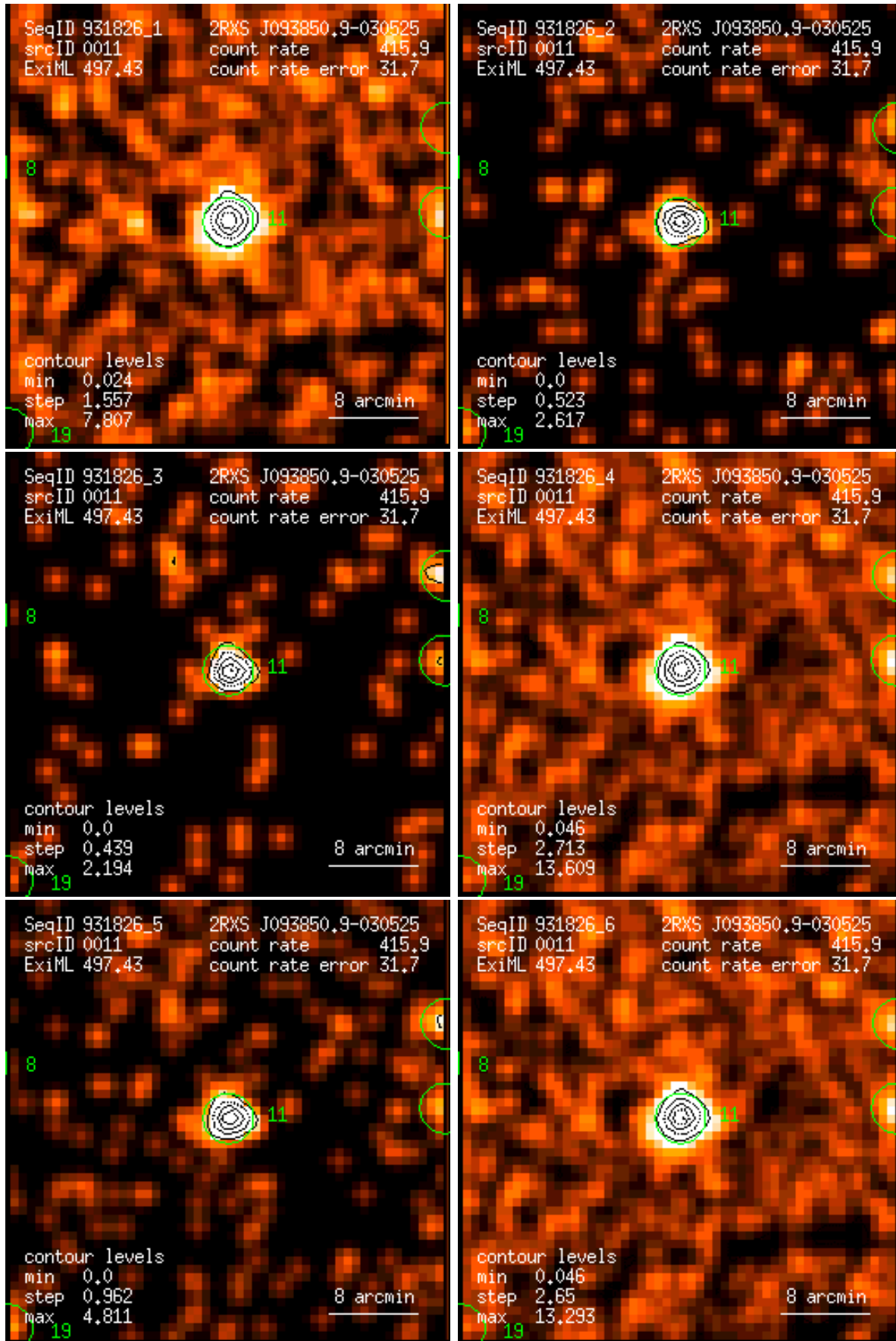
Figure 11: RASS 931826: detection 0011: band rate images, Gaussian filter: (1) PSPC channels 11 – 41, (2) 52 – 90, (3) 91 – 201, (4) 11 – 235, (5) 52 – 201, (6) 11 – 201. Broad band rates in counts/ks. Band rate contour levels in counts/ks/arcmin 2 .
