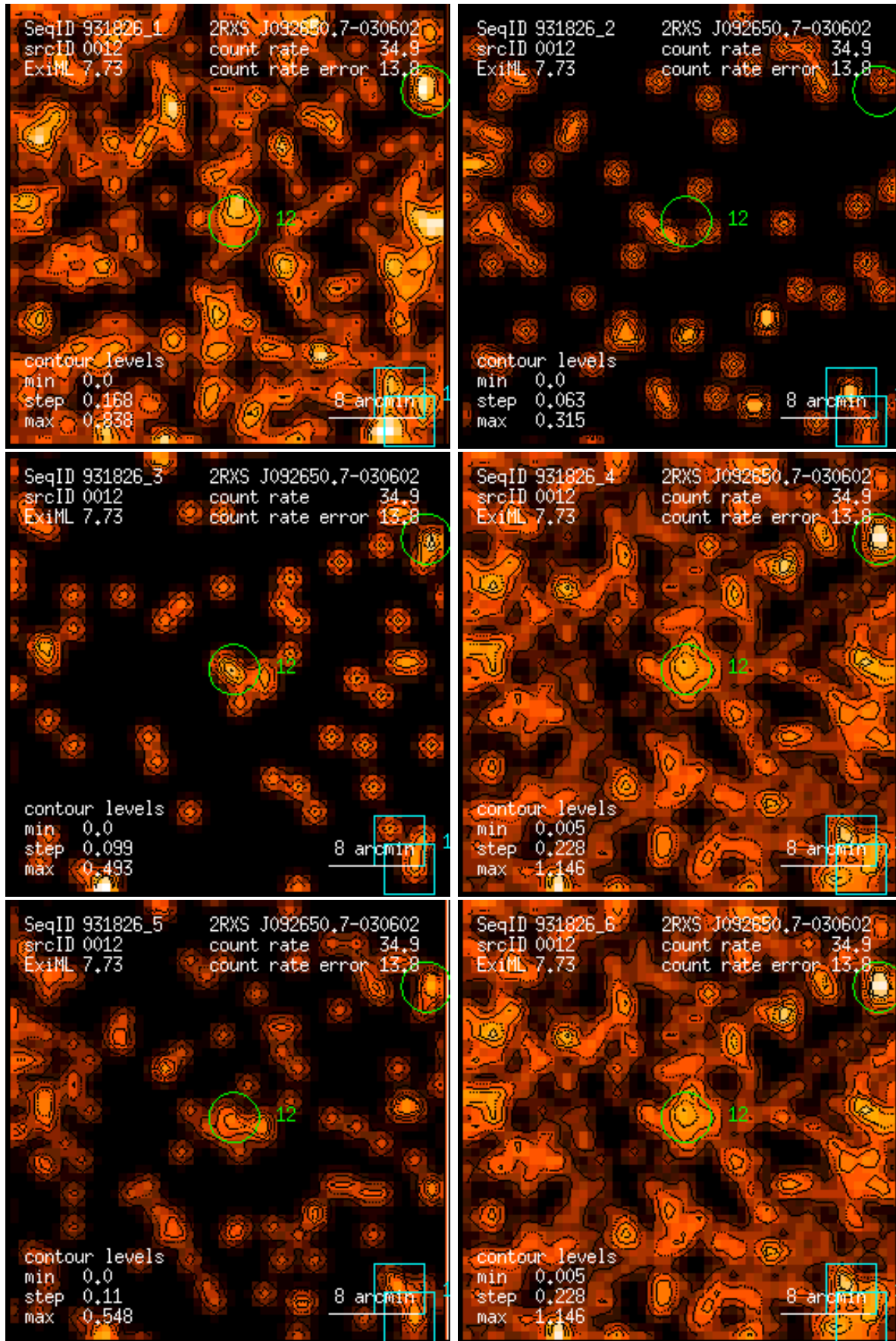
Figure 12: RASS 931826: detection 0012: band rate images, Gaussian filter: (1) PSPC channels 11 – 41, (2) 52 – 90, (3) 91 – 201, (4) 11 – 235, (5) 52 – 201, (6) 11 – 201. Broad band rates in counts/ks. Band rate contour levels in counts/ks/arcmin 2 .
