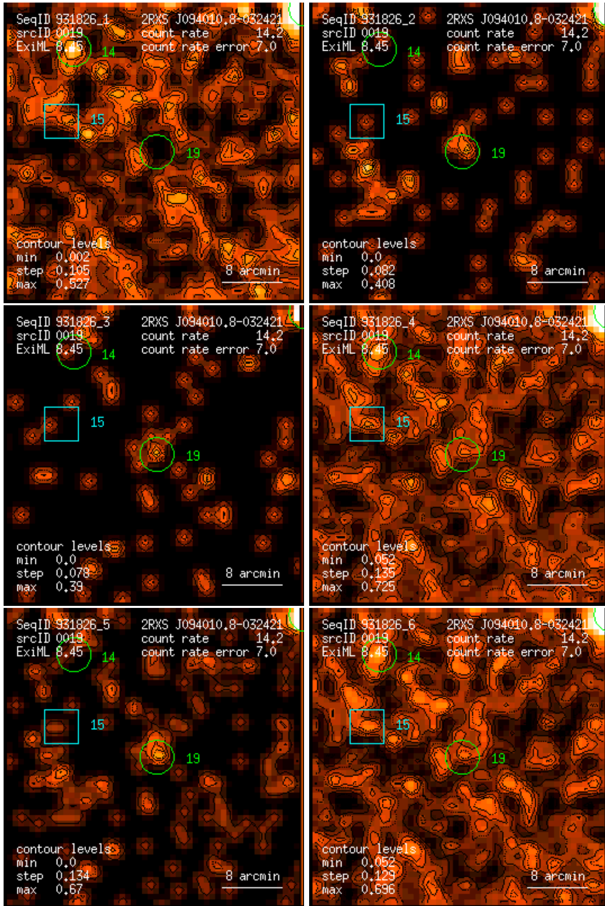
Figure 19: RASS 931826: detection 0019: band rate images, Gaussian filter: (1) PSPC channels 11 – 41, (2) 52 – 90, (3) 91 – 201, (4) 11 – 235, (5) 52 – 201, (6) 11 – 201. Broad band rates in counts/ks. Band rate contour levels in counts/ks/arcmin 2 .
