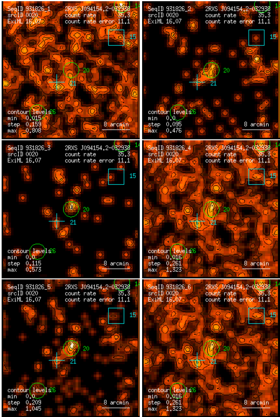
Figure 20: RASS 931826: detection 0020: band rate images, Gaussian filter: (1) PSPC channels 11 – 41, (2) 52 – 90, (3) 91 – 201, (4) 11 – 235, (5) 52 – 201, (6) 11 – 201. Broad band rates in counts/ks. Band rate contour levels in counts/ks/arcmin 2 .
