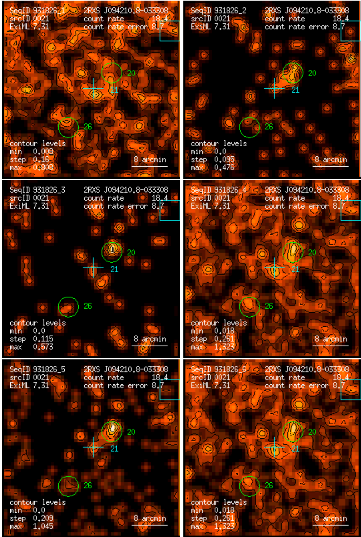
Figure 21: RASS 931826: detection 0021: band rate images, Gaussian filter: (1) PSPC channels 11 – 41, (2) 52 – 90, (3) 91 – 201, (4) 11 – 235, (5) 52 – 201, (6) 11 – 201. Broad band rates in counts/ks. Band rate contour levels in counts/ks/arcmin 2 .
